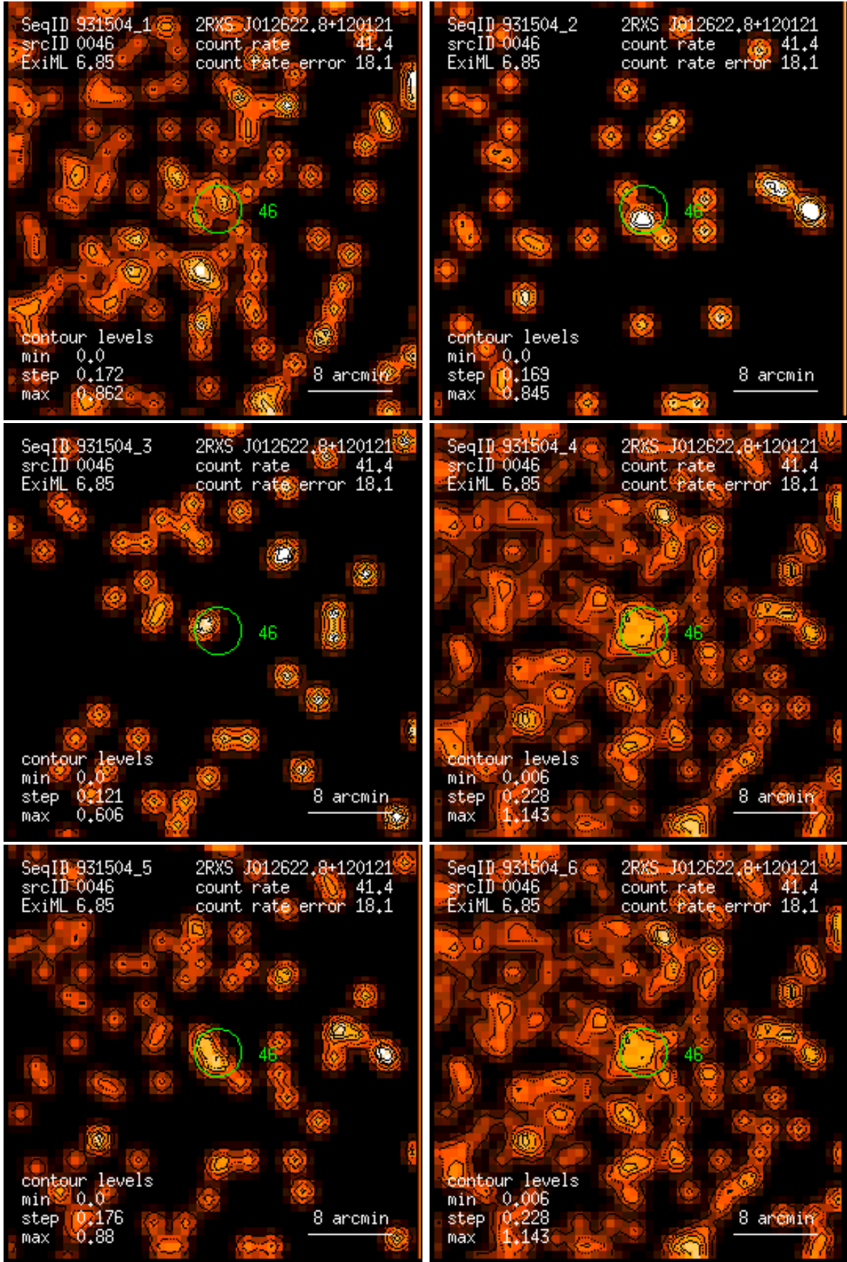
Figure 46: RASS 931504: detection 0046: band rate images, Gaussian filter: (1) PSPC channels 11 – 41, (2) 52 – 90, (3) 91 – 201, (4) 11 – 235, (5) 52 – 201, (6) 11 – 201. Broad band rates in counts/ks. Band rate contour levels in counts/ks/arcmin 2 .
