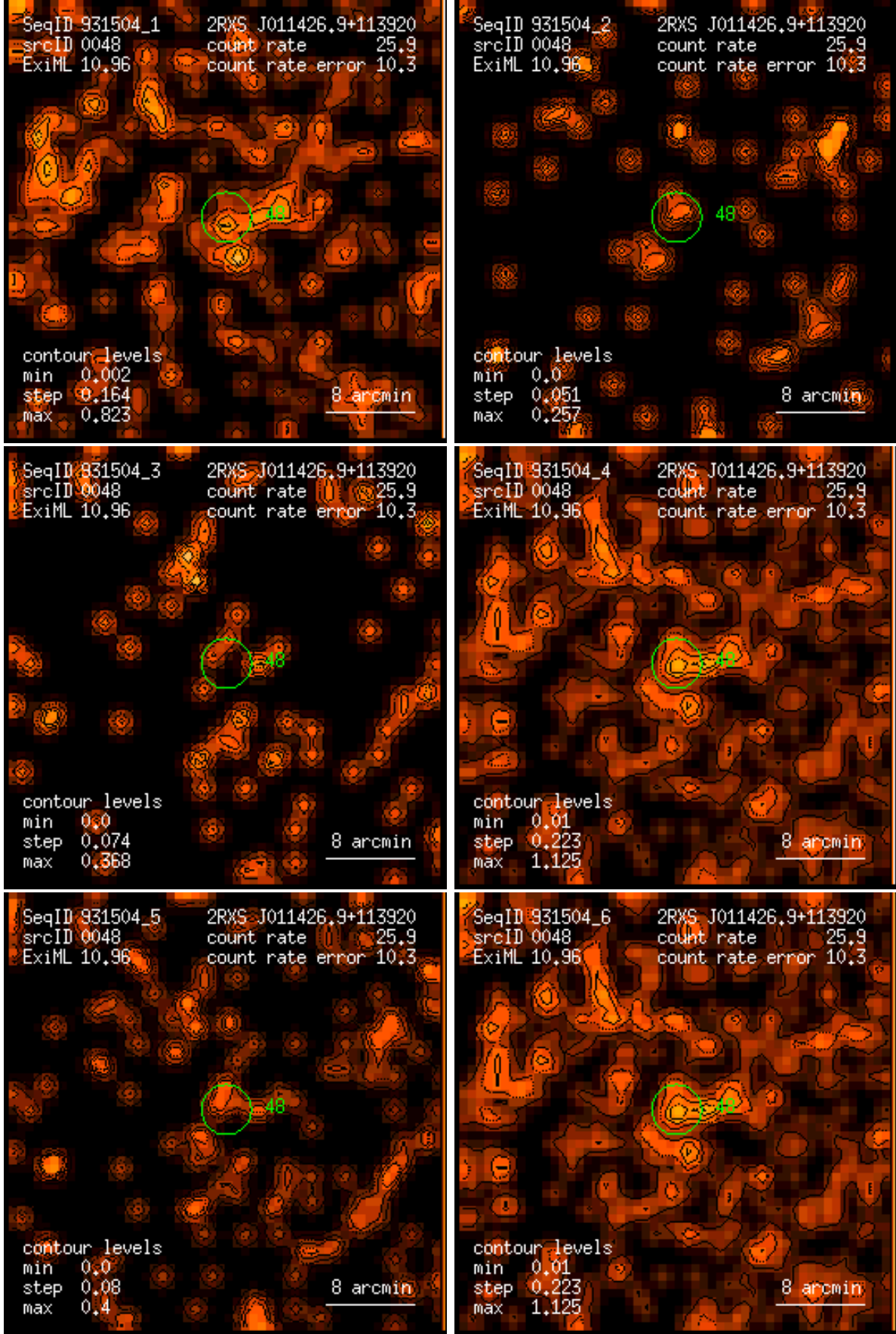
Figure 48: RASS 931504: detection 0048: band rate images, Gaussian filter: (1) PSPC channels 11 – 41, (2) 52 – 90, (3) 91 – 201, (4) 11 – 235, (5) 52 – 201, (6) 11 – 201. Broad band rates in counts/ks. Band rate contour levels in counts/ks/arcmin 2 .
