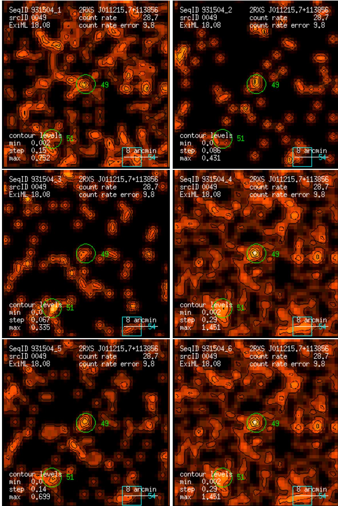
Figure 49: RASS 931504: detection 0049: band rate images, Gaussian filter: (1) PSPC channels 11 – 41, (2) 52 – 90, (3) 91 – 201, (4) 11 – 235, (5) 52 – 201, (6) 11 – 201. Broad band rates in counts/ks. Band rate contour levels in counts/ks/arcmin 2 .
