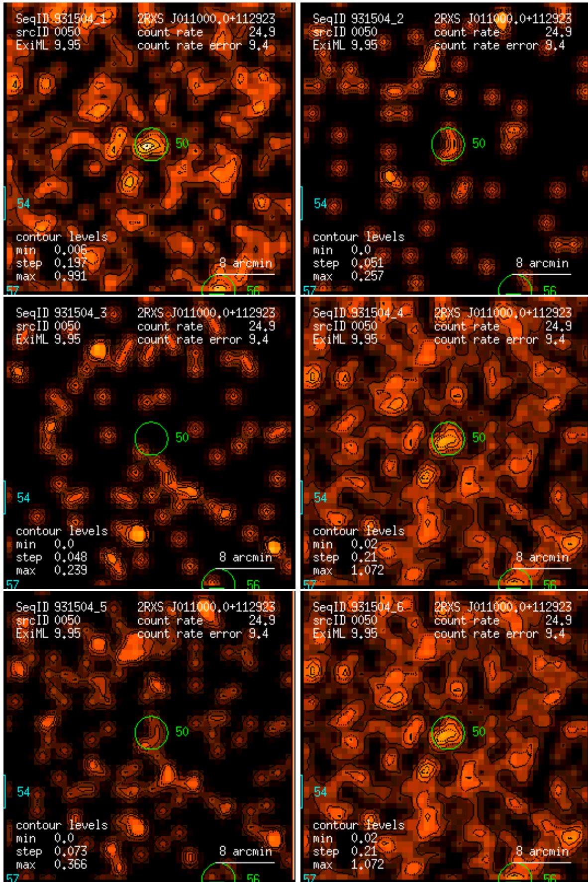
Figure 50: RASS 931504: detection 0050: band rate images, Gaussian filter: (1) PSPC channels 11 – 41, (2) 52 – 90, (3) 91 – 201, (4) 11 – 235, (5) 52 – 201, (6) 11 – 201. Broad band rates in counts/ks. Band rate contour levels in counts/ks/arcmin 2 .
