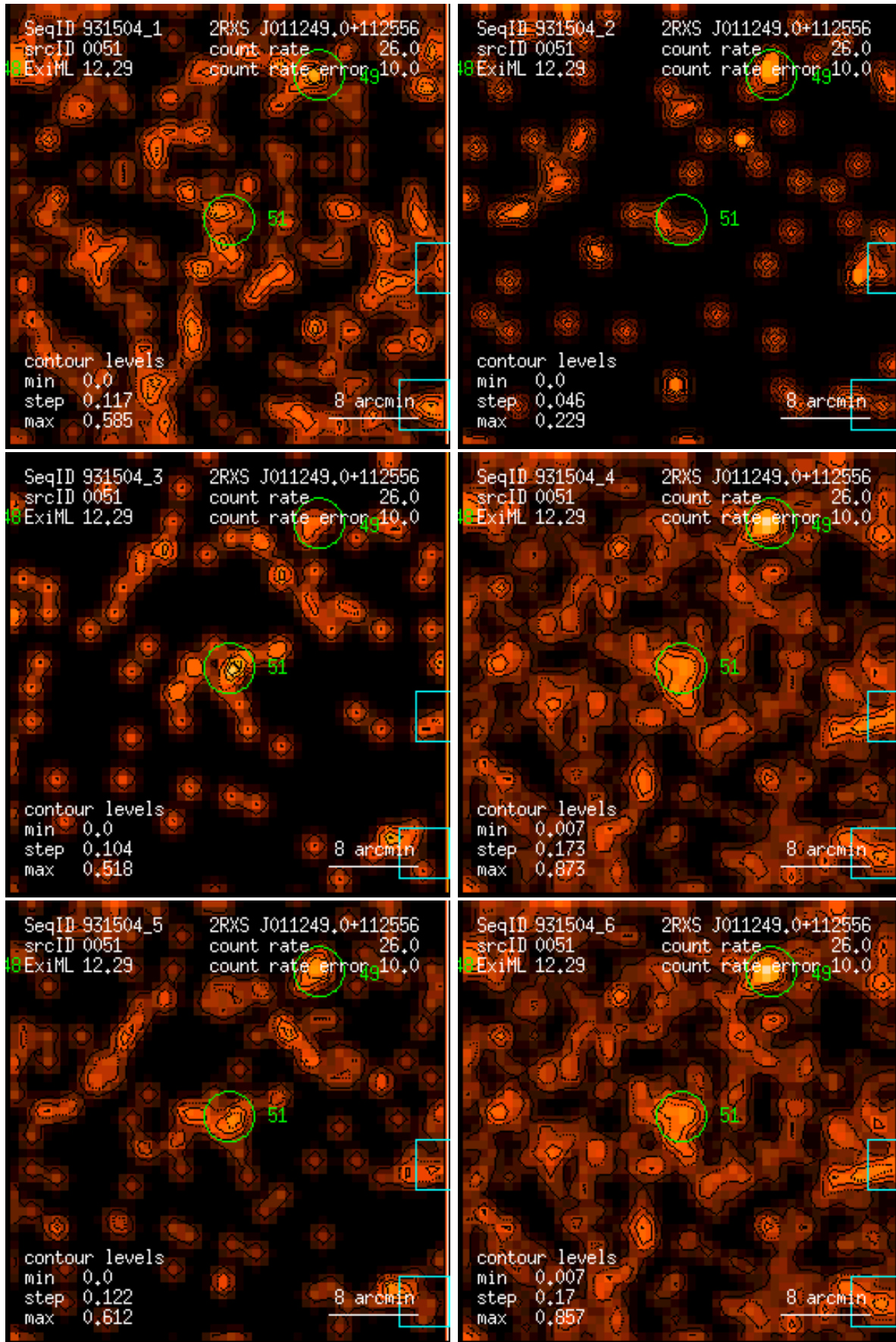
Figure 51: RASS 931504: detection 0051: band rate images, Gaussian filter: (1) PSPC channels 11 – 41, (2) 52 – 90, (3) 91 – 201, (4) 11 – 235, (5) 52 – 201, (6) 11 – 201. Broad band rates in counts/ks. Band rate contour levels in counts/ks/arcmin 2 .
