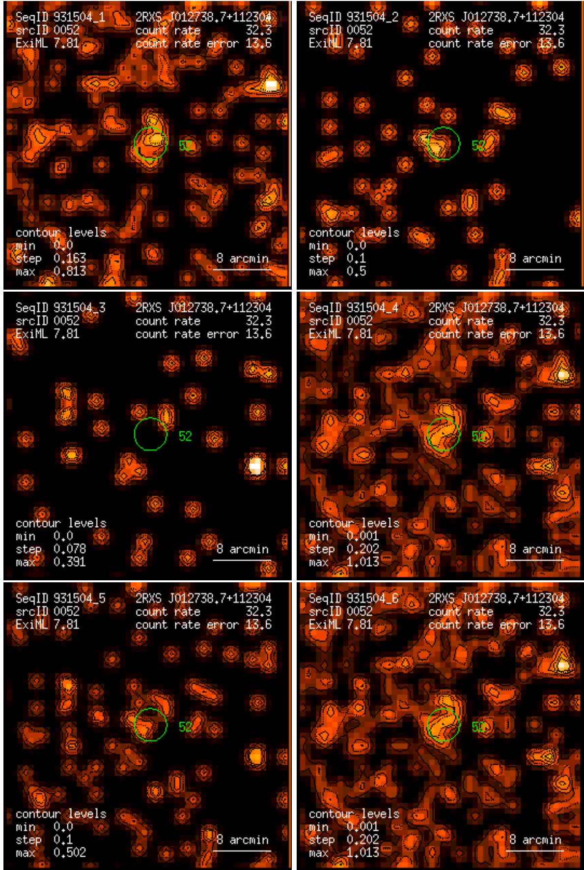
Figure 52: RASS 931504: detection 0052: band rate images, Gaussian filter: (1) PSPC channels 11 – 41, (2) 52 – 90, (3) 91 – 201, (4) 11 – 235, (5) 52 – 201, (6) 11 – 201. Broad band rates in counts/ks. Band rate contour levels in counts/ks/arcmin 2 .
