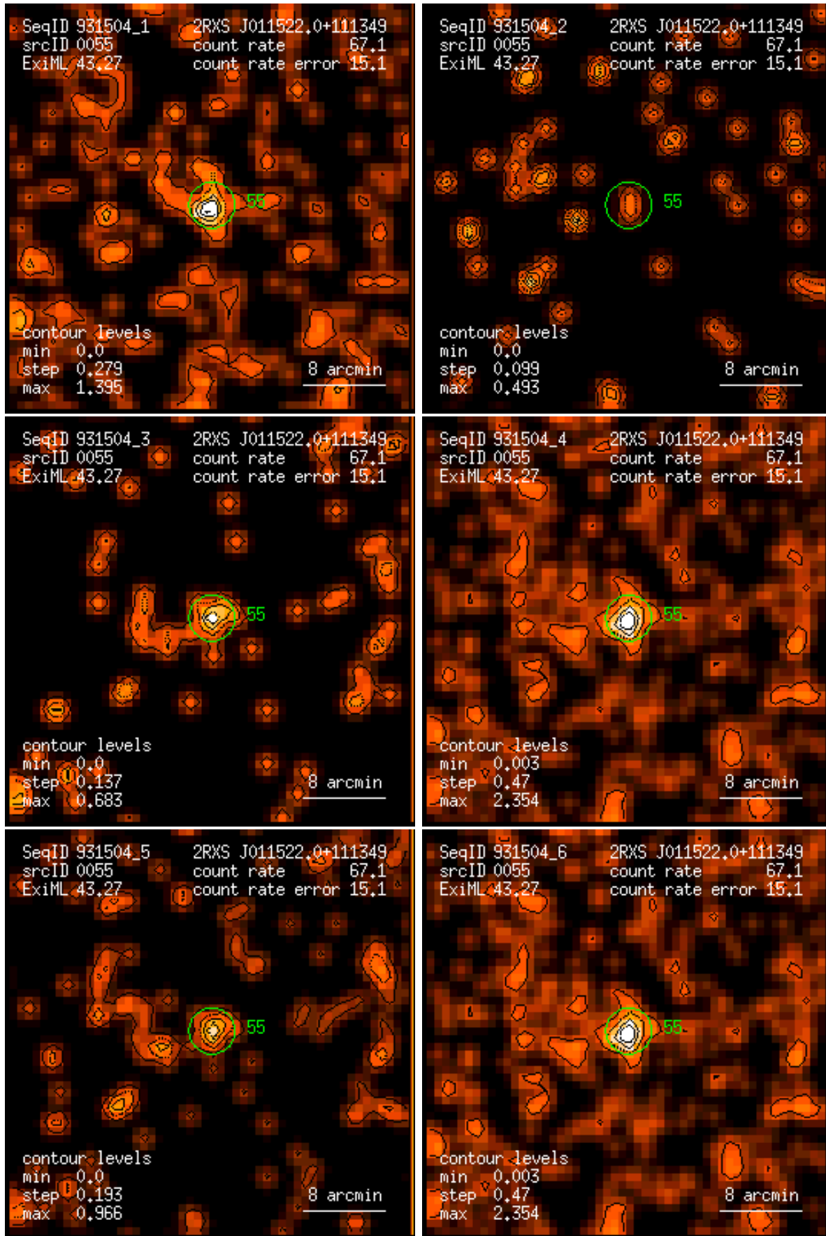
Figure 55: RASS 931504: detection 0055: band rate images, Gaussian filter: (1) PSPC channels 11 – 41, (2) 52 – 90, (3) 91 – 201, (4) 11 – 235, (5) 52 – 201, (6) 11 – 201. Broad band rates in counts/ks. Band rate contour levels in counts/ks/arcmin 2 .
