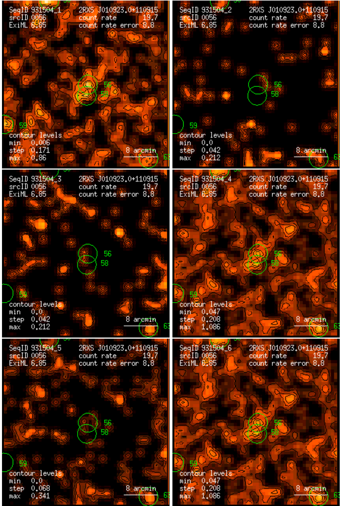
Figure 56: RASS 931504: detection 0056: band rate images, Gaussian filter: (1) PSPC channels 11 – 41, (2) 52 – 90, (3) 91 – 201, (4) 11 – 235, (5) 52 – 201, (6) 11 – 201. Broad band rates in counts/ks. Band rate contour levels in counts/ks/arcmin 2 .
