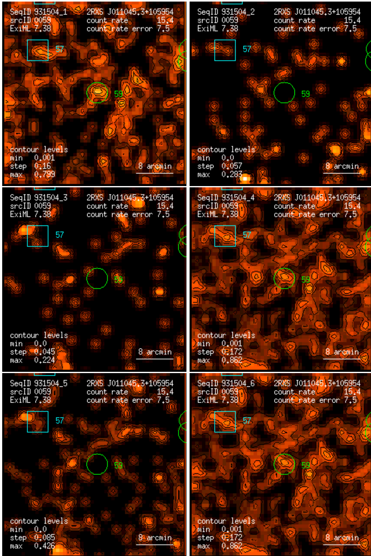
Figure 59: RASS 931504: detection 0059: band rate images, Gaussian filter: (1) PSPC channels 11 – 41, (2) 52 – 90, (3) 91 – 201, (4) 11 – 235, (5) 52 – 201, (6) 11 – 201. Broad band rates in counts/ks. Band rate contour levels in counts/ks/arcmin 2 .
