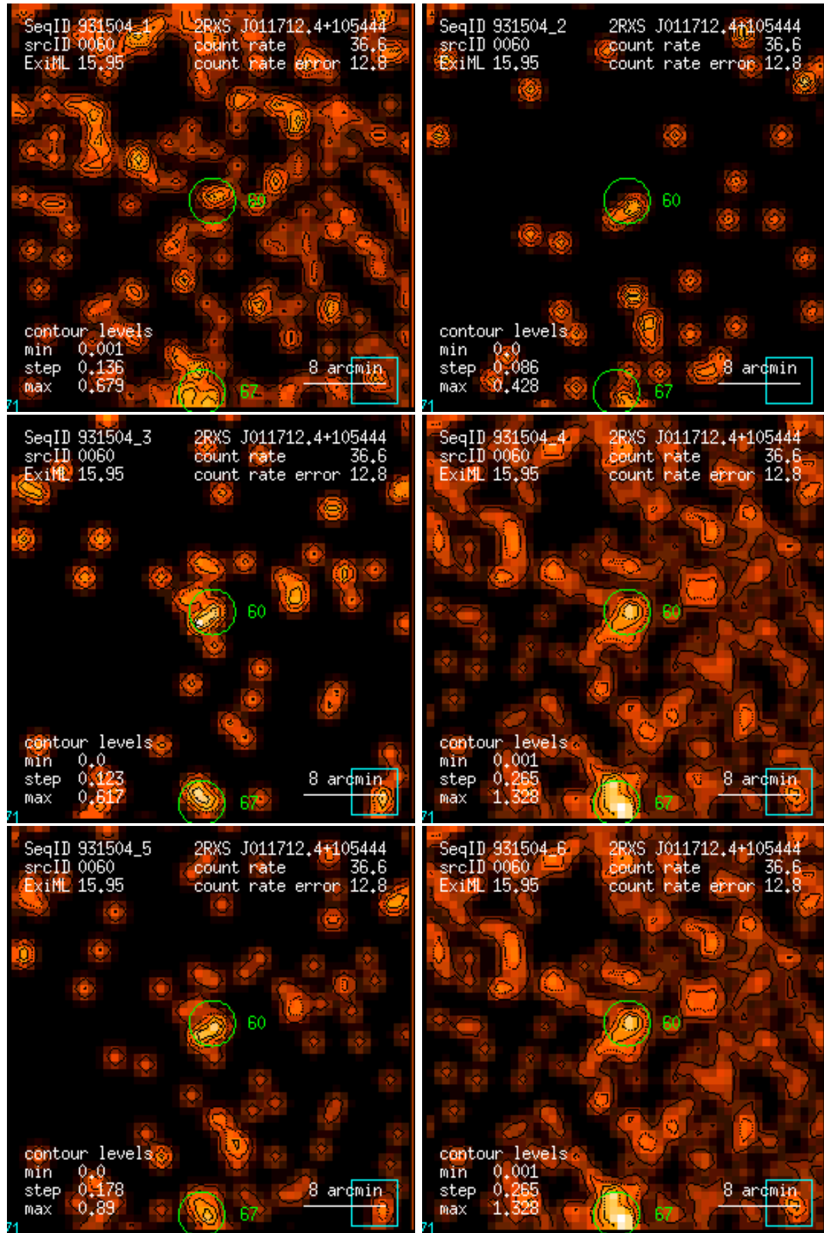
Figure 60: RASS 931504: detection 0060: band rate images, Gaussian filter: (1) PSPC channels 11 – 41, (2) 52 – 90, (3) 91 – 201, (4) 11 – 235, (5) 52 – 201, (6) 11 – 201. Broad band rates in counts/ks. Band rate contour levels in counts/ks/arcmin 2 .
