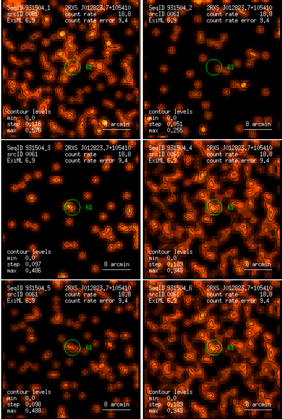
Figure 61: RASS 931504: detection 0061: band rate images, Gaussian filter: (1) PSPC channels 11 – 41, (2) 52 – 90, (3) 91 – 201, (4) 11 – 235, (5) 52 – 201, (6) 11 – 201. Broad band rates in counts/ks. Band rate contour levels in counts/ks/arcmin 2 .
