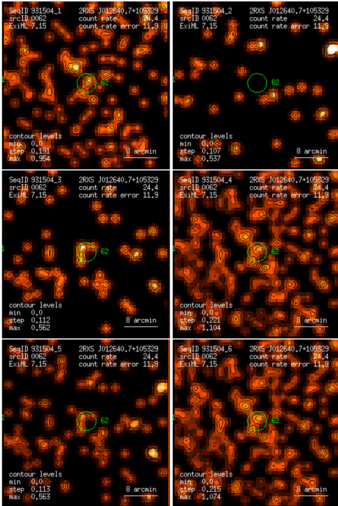
Figure 62: RASS 931504: detection 0062: band rate images, Gaussian filter: (1) PSPC channels 11 – 41, (2) 52 – 90, (3) 91 – 201, (4) 11 – 235, (5) 52 – 201, (6) 11 – 201. Broad band rates in counts/ks. Band rate contour levels in counts/ks/arcmin 2 .
