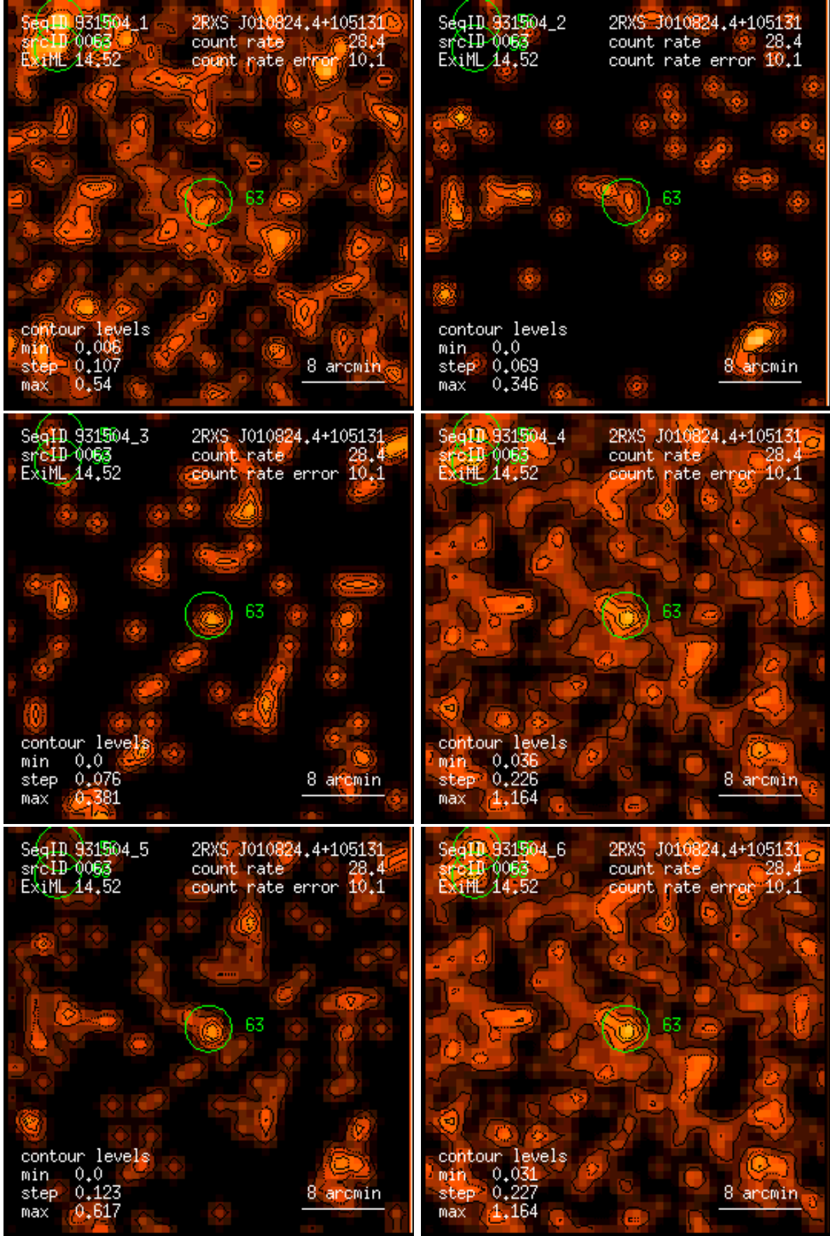
Figure 63: RASS 931504: detection 0063: band rate images, Gaussian filter: (1) PSPC channels 11 – 41, (2) 52 – 90, (3) 91 – 201, (4) 11 – 235, (5) 52 – 201, (6) 11 – 201. Broad band rates in counts/ks. Band rate contour levels in counts/ks/arcmin 2 .
