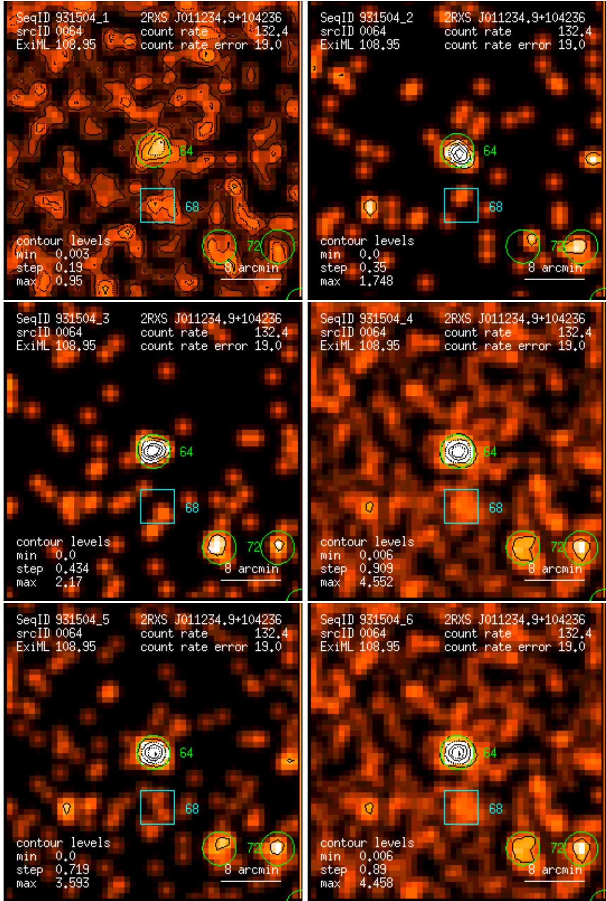
Figure 64: RASS 931504: detection 0064: band rate images, Gaussian filter: (1) PSPC channels 11 – 41, (2) 52 – 90, (3) 91 – 201, (4) 11 – 235, (5) 52 – 201, (6) 11 – 201. Broad band rates in counts/ks. Band rate contour levels in counts/ks/arcmin 2 .
