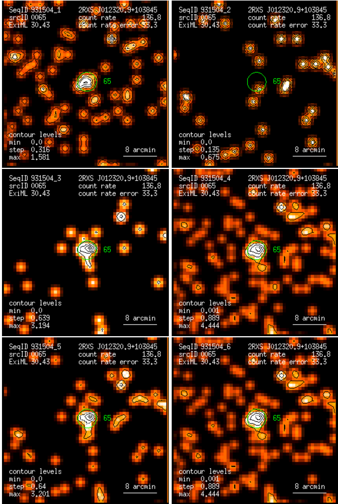
Figure 65: RASS 931504: detection 0065: band rate images, Gaussian filter: (1) PSPC channels 11 – 41, (2) 52 – 90, (3) 91 – 201, (4) 11 – 235, (5) 52 – 201, (6) 11 – 201. Broad band rates in counts/ks. Band rate contour levels in counts/ks/arcmin 2 .
