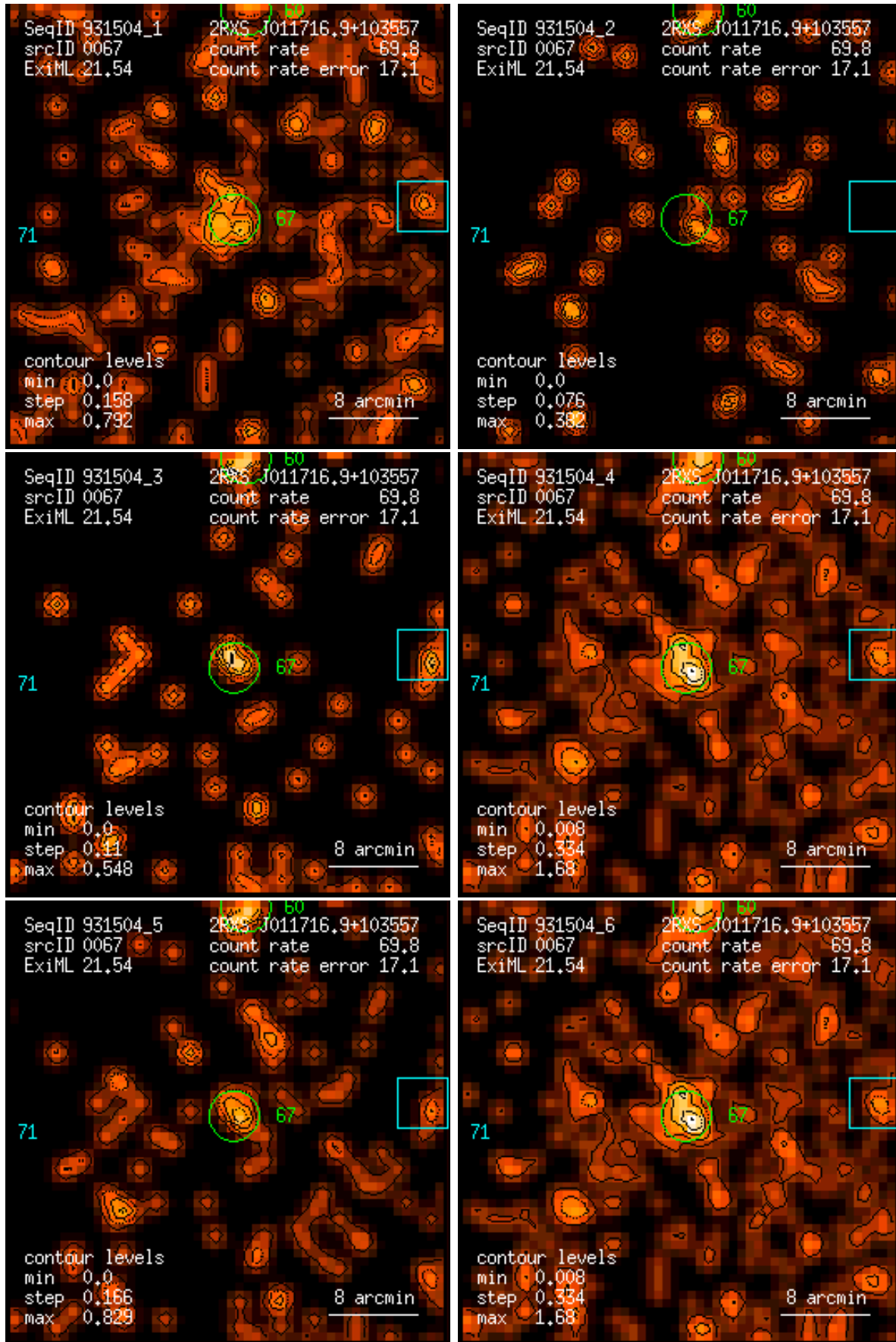
Figure 67: RASS 931504: detection 0067: band rate images, Gaussian filter: (1) PSPC channels 11 – 41, (2) 52 – 90, (3) 91 – 201, (4) 11 – 235, (5) 52 – 201, (6) 11 – 201. Broad band rates in counts/ks. Band rate contour levels in counts/ks/arcmin 2 .
