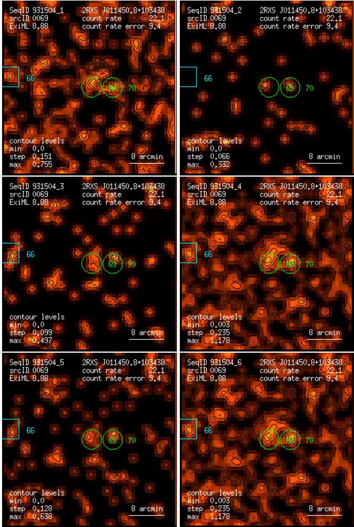
Figure 69: RASS 931504: detection 0069: band rate images, Gaussian filter: (1) PSPC channels 11 – 41, (2) 52 – 90, (3) 91 – 201, (4) 11 – 235, (5) 52 – 201, (6) 11 – 201. Broad band rates in counts/ks. Band rate contour levels in counts/ks/arcmin 2 .
