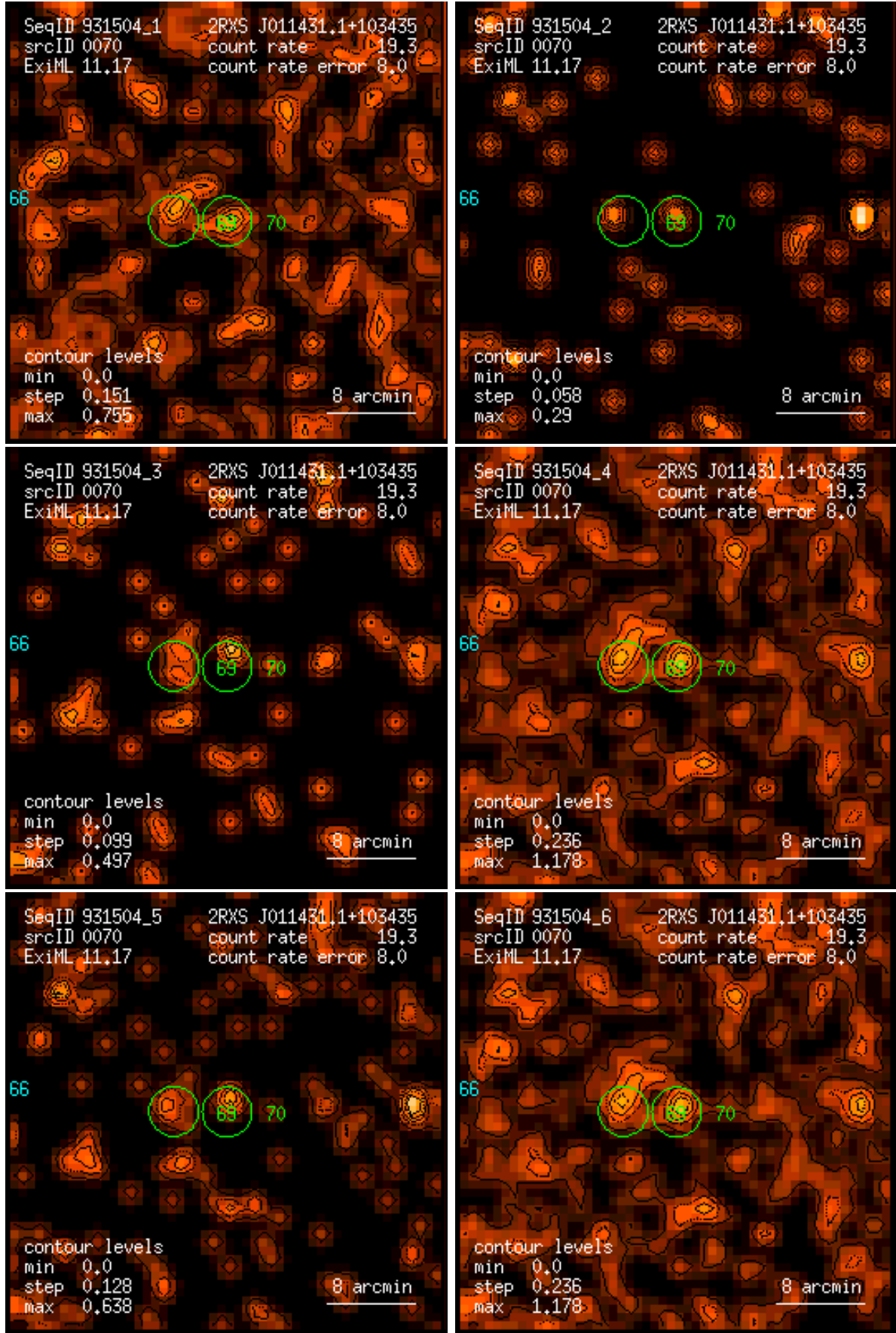
Figure 70: RASS 931504: detection 0070: band rate images, Gaussian filter: (1) PSPC channels 11 – 41, (2) 52 – 90, (3) 91 – 201, (4) 11 – 235, (5) 52 – 201, (6) 11 – 201. Broad band rates in counts/ks. Band rate contour levels in counts/ks/arcmin 2 .
