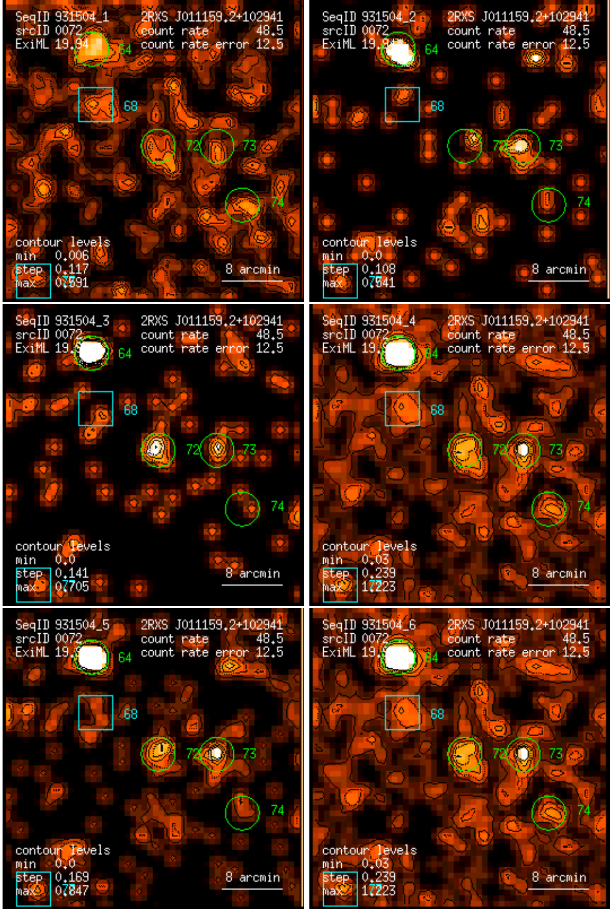
Figure 72: RASS 931504: detection 0072: band rate images, Gaussian filter: (1) PSPC channels 11 – 41, (2) 52 – 90, (3) 91 – 201, (4) 11 – 235, (5) 52 – 201, (6) 11 – 201. Broad band rates in counts/ks. Band rate contour levels in counts/ks/arcmin 2 .
