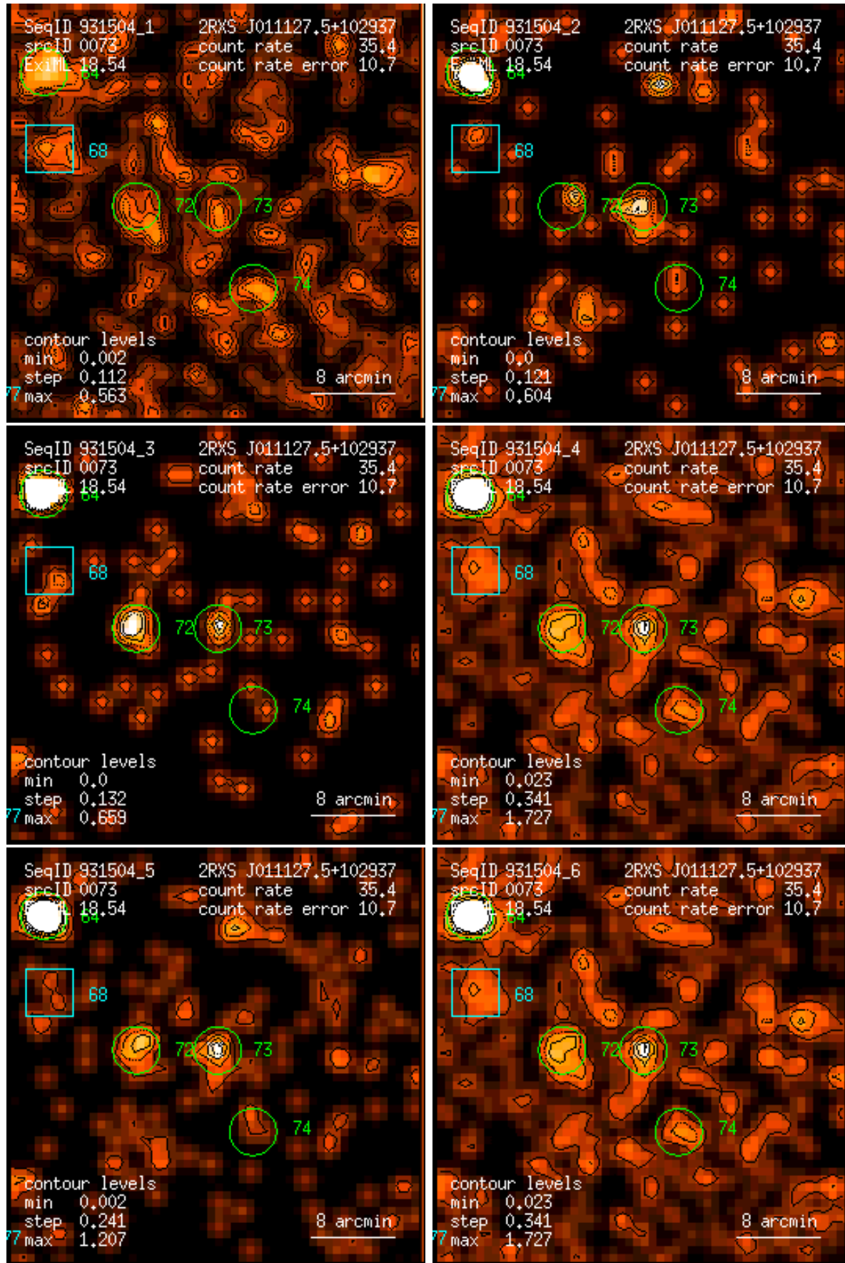
Figure 73: RASS 931504: detection 0073: band rate images, Gaussian filter: (1) PSPC channels 11 – 41, (2) 52 – 90, (3) 91 – 201, (4) 11 – 235, (5) 52 – 201, (6) 11 – 201. Broad band rates in counts/ks. Band rate contour levels in counts/ks/arcmin 2 .
