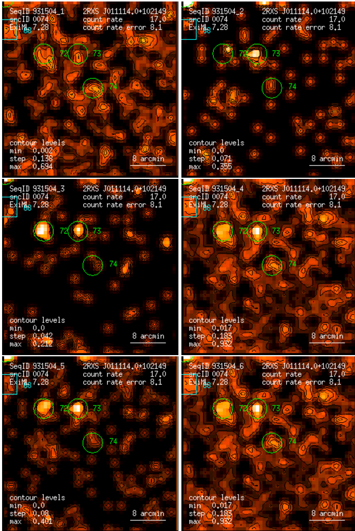
Figure 74: RASS 931504: detection 0074: band rate images, Gaussian filter: (1) PSPC channels 11 – 41, (2) 52 – 90, (3) 91 – 201, (4) 11 – 235, (5) 52 – 201, (6) 11 – 201. Broad band rates in counts/ks. Band rate contour levels in counts/ks/arcmin 2 .
