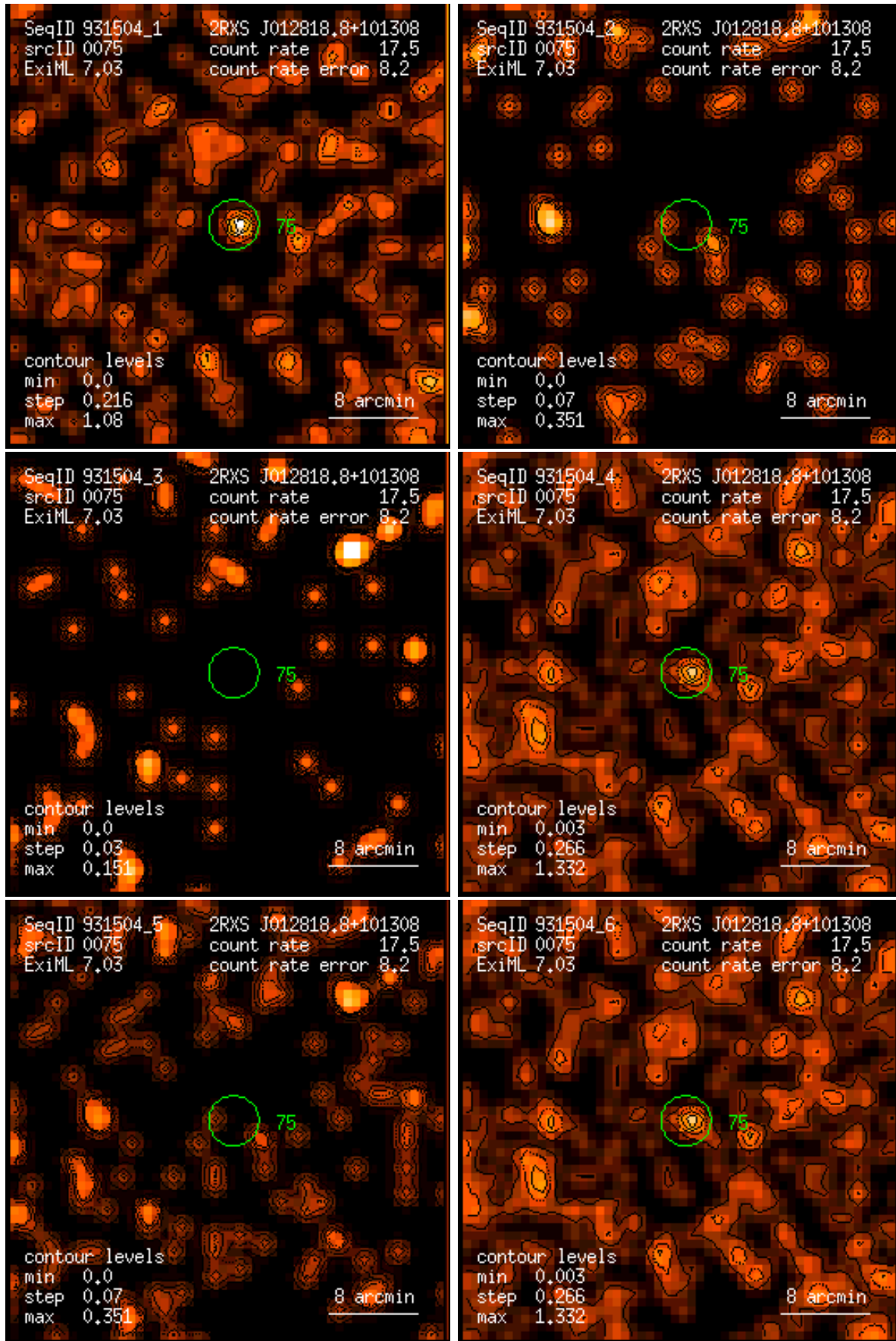
Figure 75: RASS 931504: detection 0075: band rate images, Gaussian filter: (1) PSPC channels 11 – 41, (2) 52 – 90, (3) 91 – 201, (4) 11 – 235, (5) 52 – 201, (6) 11 – 201. Broad band rates in counts/ks. Band rate contour levels in counts/ks/arcmin 2 .
