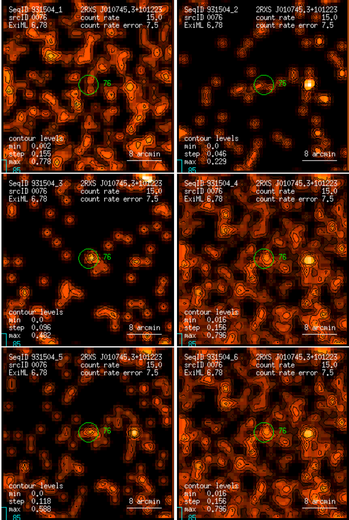
Figure 76: RASS 931504: detection 0076: band rate images, Gaussian filter: (1) PSPC channels 11 – 41, (2) 52 – 90, (3) 91 – 201, (4) 11 – 235, (5) 52 – 201, (6) 11 – 201. Broad band rates in counts/ks. Band rate contour levels in counts/ks/arcmin 2 .
