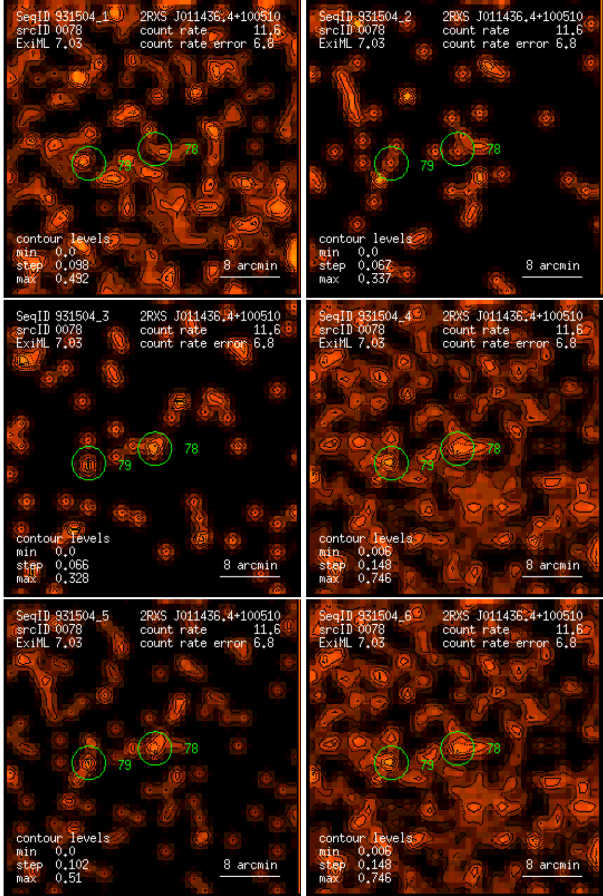
Figure 78: RASS 931504: detection 0078: band rate images, Gaussian filter: (1) PSPC channels 11 – 41, (2) 52 – 90, (3) 91 – 201, (4) 11 – 235, (5) 52 – 201, (6) 11 – 201. Broad band rates in counts/ks. Band rate contour levels in counts/ks/arcmin 2 .
