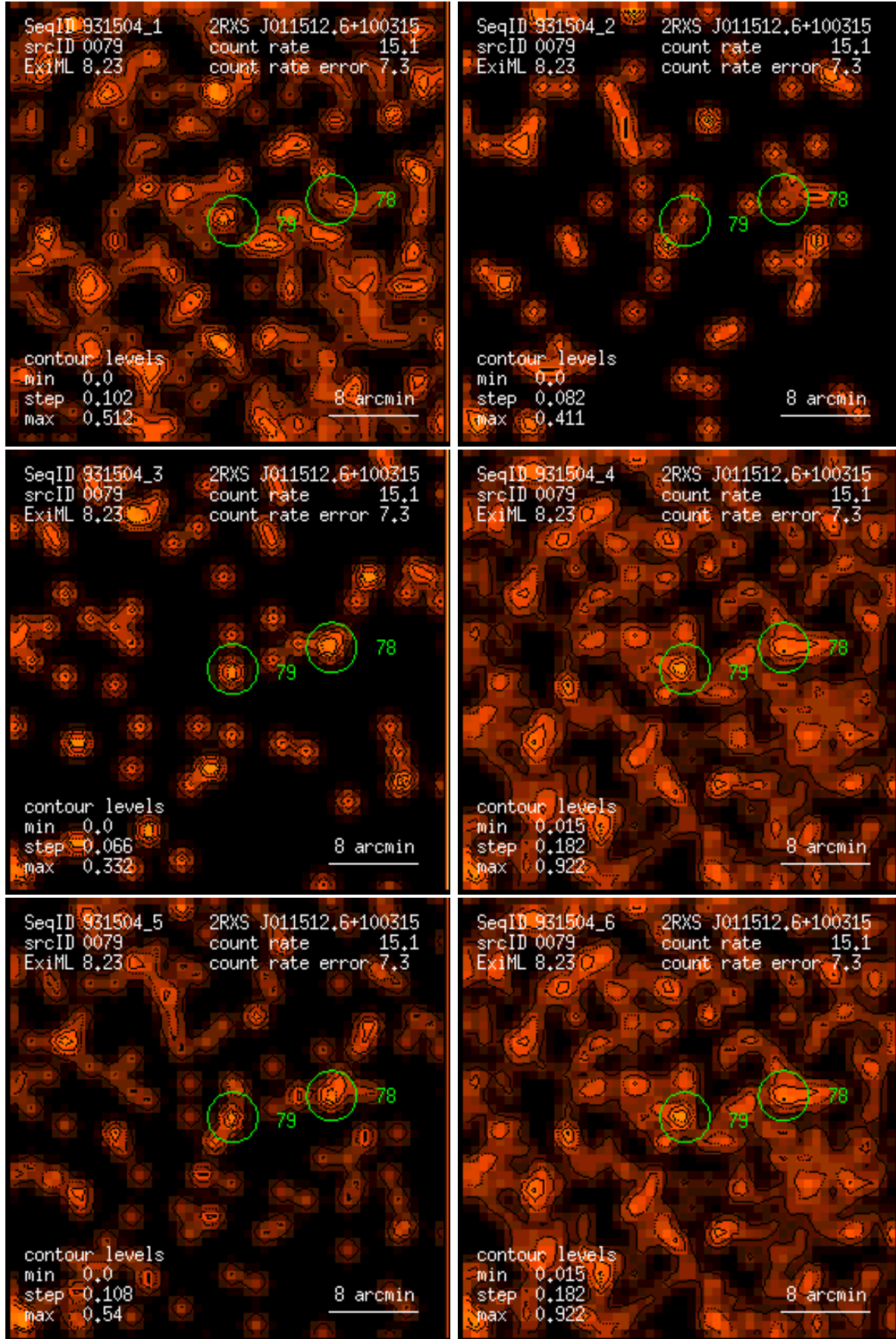
Figure 79: RASS 931504: detection 0079: band rate images, Gaussian filter: (1) PSPC channels 11 – 41, (2) 52 – 90, (3) 91 – 201, (4) 11 – 235, (5) 52 – 201, (6) 11 – 201. Broad band rates in counts/ks. Band rate contour levels in counts/ks/arcmin 2 .
