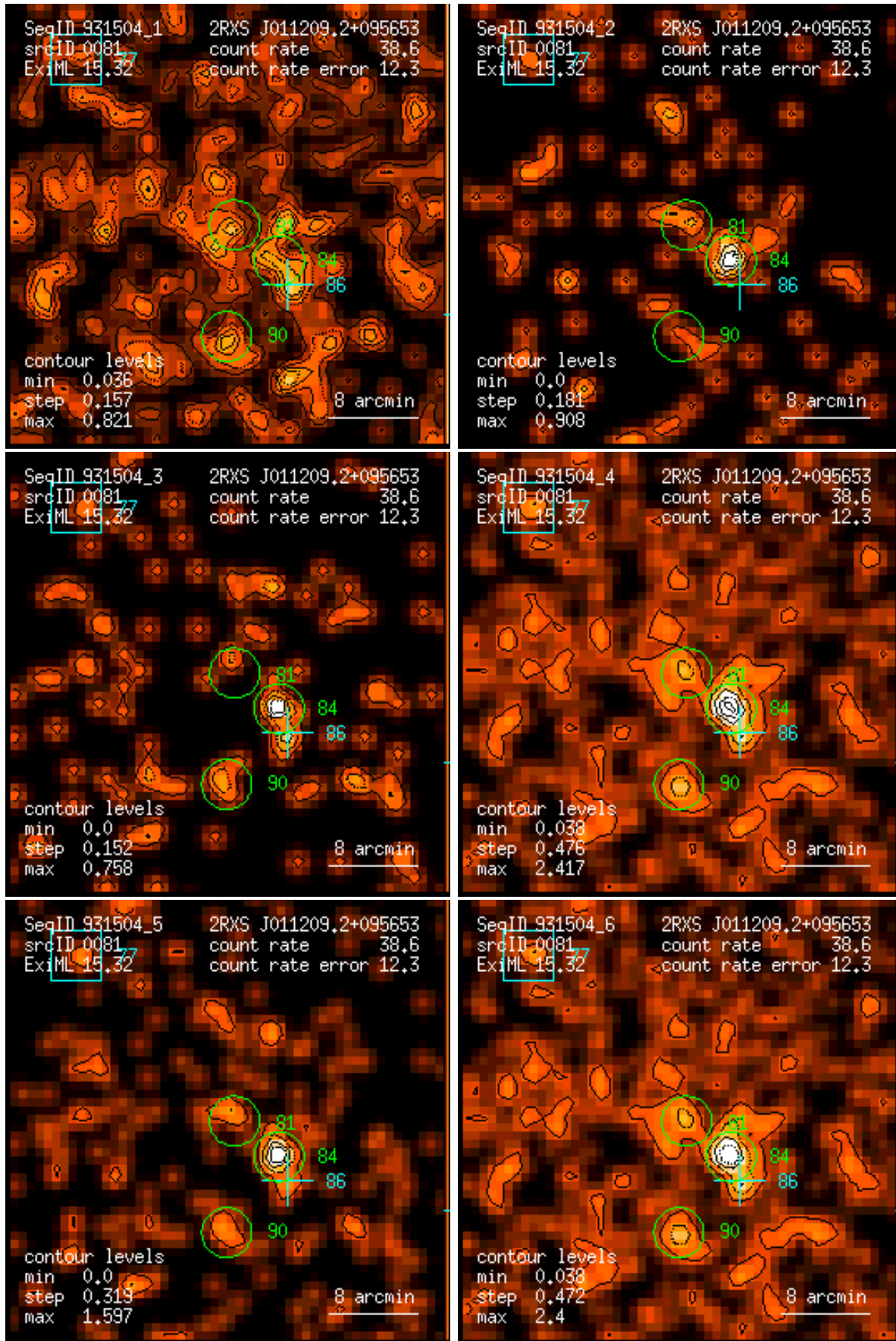
Figure 81: RASS 931504: detection 0081: band rate images, Gaussian filter: (1) PSPC channels 11 – 41, (2) 52 – 90, (3) 91 – 201, (4) 11 – 235, (5) 52 – 201, (6) 11 – 201. Broad band rates in counts/ks. Band rate contour levels in counts/ks/arcmin 2 .
