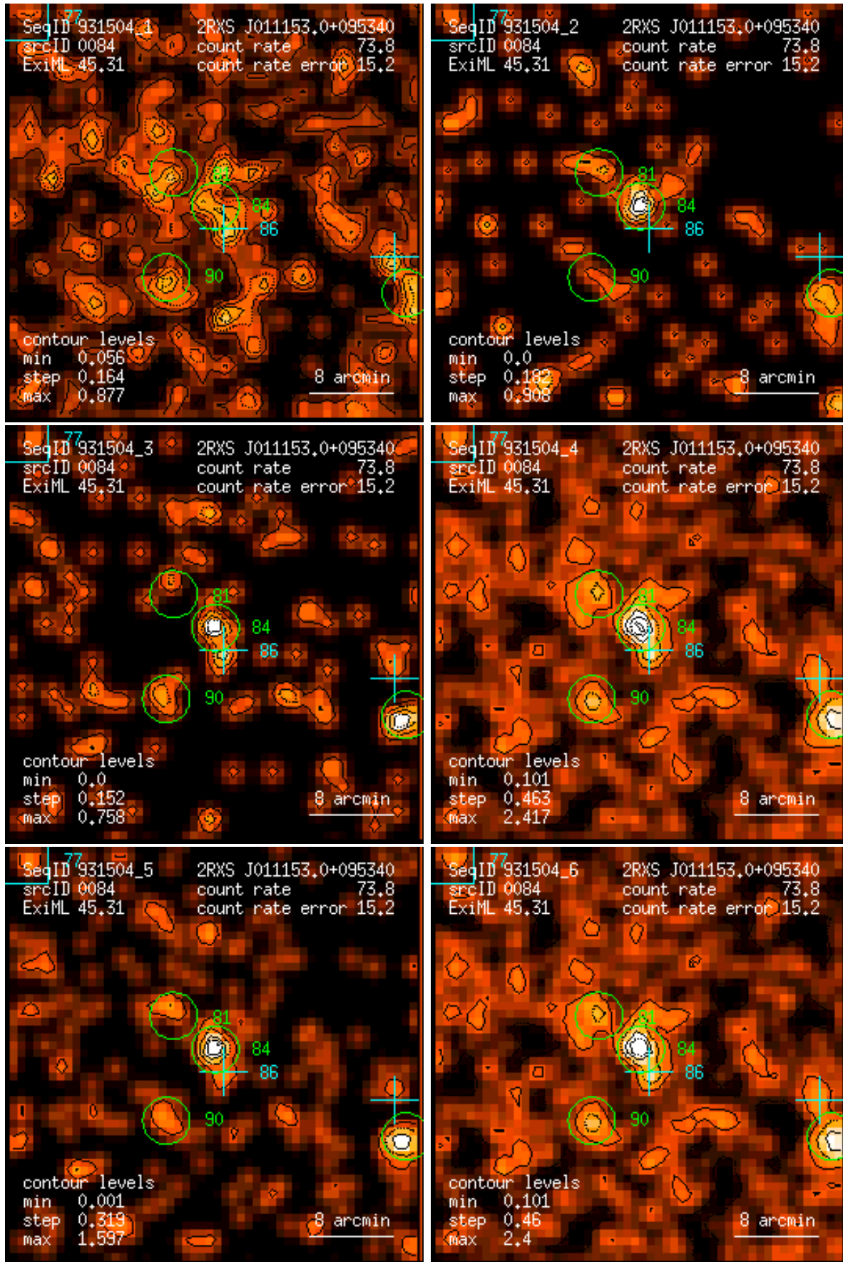
Figure 84: RASS 931504: detection 0084: band rate images, Gaussian filter: (1) PSPC channels 11 – 41, (2) 52 – 90, (3) 91 – 201, (4) 11 – 235, (5) 52 – 201, (6) 11 – 201. Broad band rates in counts/ks. Band rate contour levels in counts/ks/arcmin 2 .
