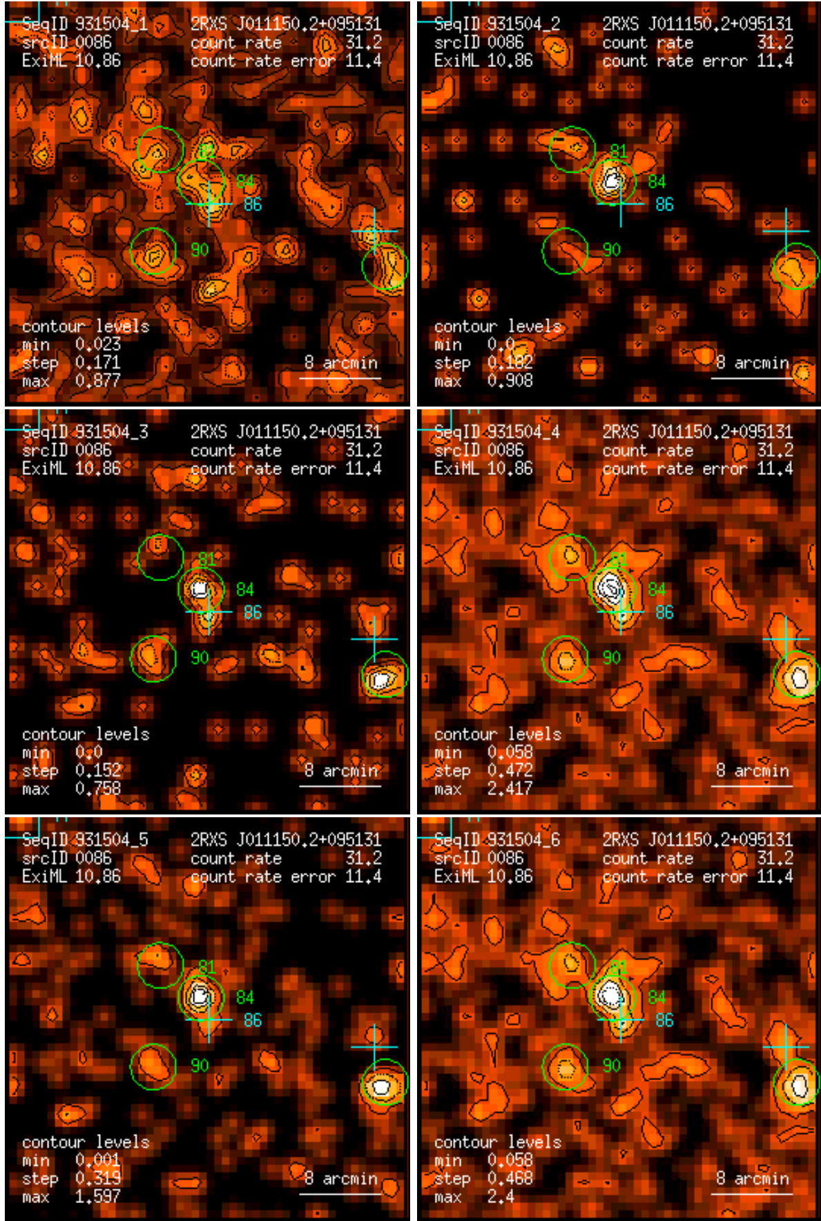
Figure 86: RASS 931504: detection 0086: band rate images, Gaussian filter: (1) PSPC channels 11 – 41, (2) 52 – 90, (3) 91 – 201, (4) 11 – 235, (5) 52 – 201, (6) 11 – 201. Broad band rates in counts/ks. Band rate contour levels in counts/ks/arcmin 2 .
