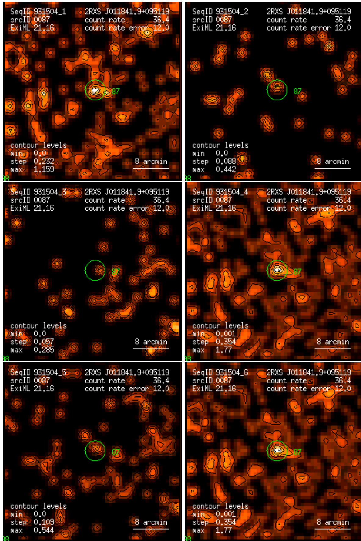
Figure 87: RASS 931504: detection 0087: band rate images, Gaussian filter: (1) PSPC channels 11 – 41, (2) 52 – 90, (3) 91 – 201, (4) 11 – 235, (5) 52 – 201, (6) 11 – 201. Broad band rates in counts/ks. Band rate contour levels in counts/ks/arcmin 2 .
