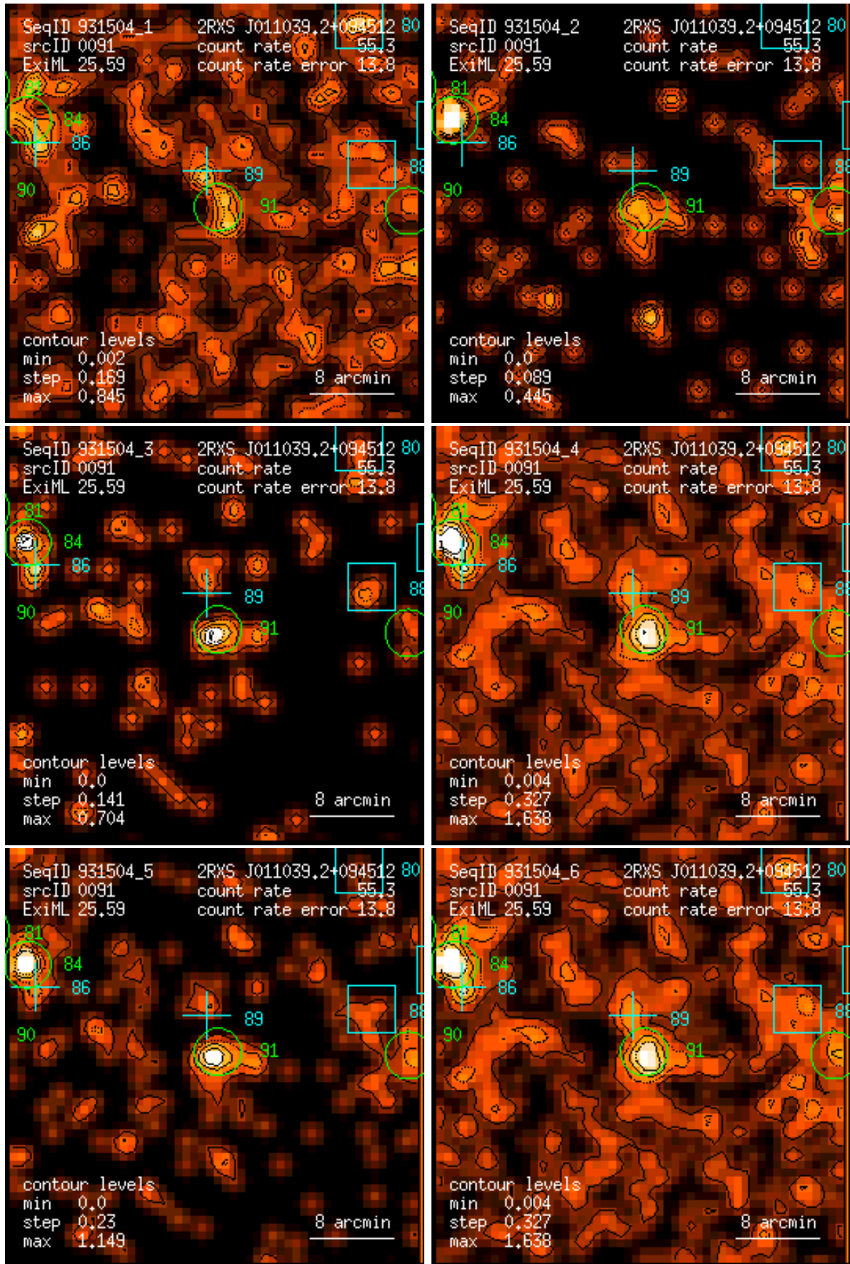
Figure 91: RASS 931504: detection 0091: band rate images, Gaussian filter: (1) PSPC channels 11 – 41, (2) 52 – 90, (3) 91 – 201, (4) 11 – 235, (5) 52 – 201, (6) 11 – 201. Broad band rates in counts/ks. Band rate contour levels in counts/ks/arcmin 2 .
