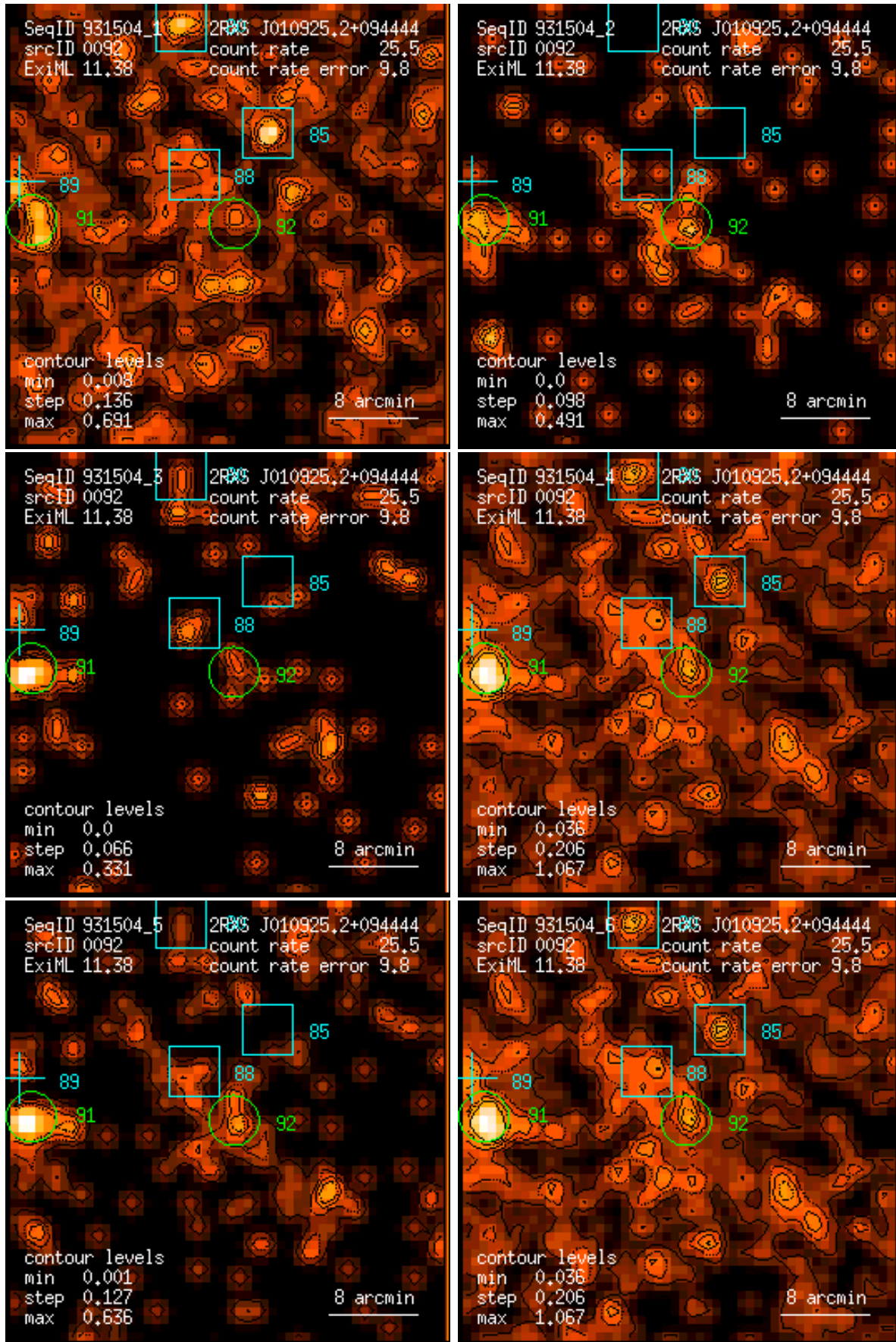
Figure 92: RASS 931504: detection 0092: band rate images, Gaussian filter: (1) PSPC channels 11 – 41, (2) 52 – 90, (3) 91 – 201, (4) 11 – 235, (5) 52 – 201, (6) 11 – 201. Broad band rates in counts/ks. Band rate contour levels in counts/ks/arcmin 2 .
