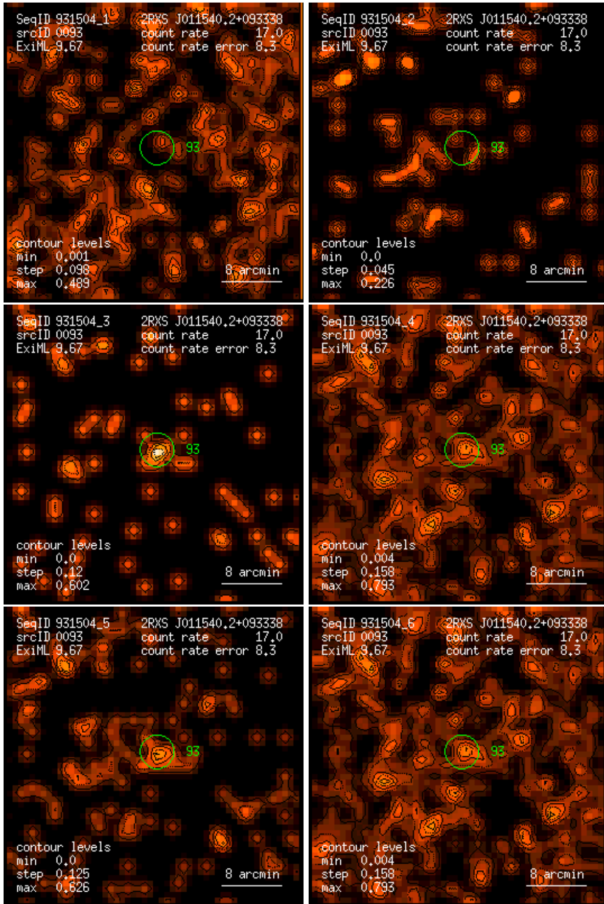
Figure 93: RASS 931504: detection 0093: band rate images, Gaussian filter: (1) PSPC channels 11 – 41, (2) 52 – 90, (3) 91 – 201, (4) 11 – 235, (5) 52 – 201, (6) 11 – 201. Broad band rates in counts/ks. Band rate contour levels in counts/ks/arcmin 2 .
