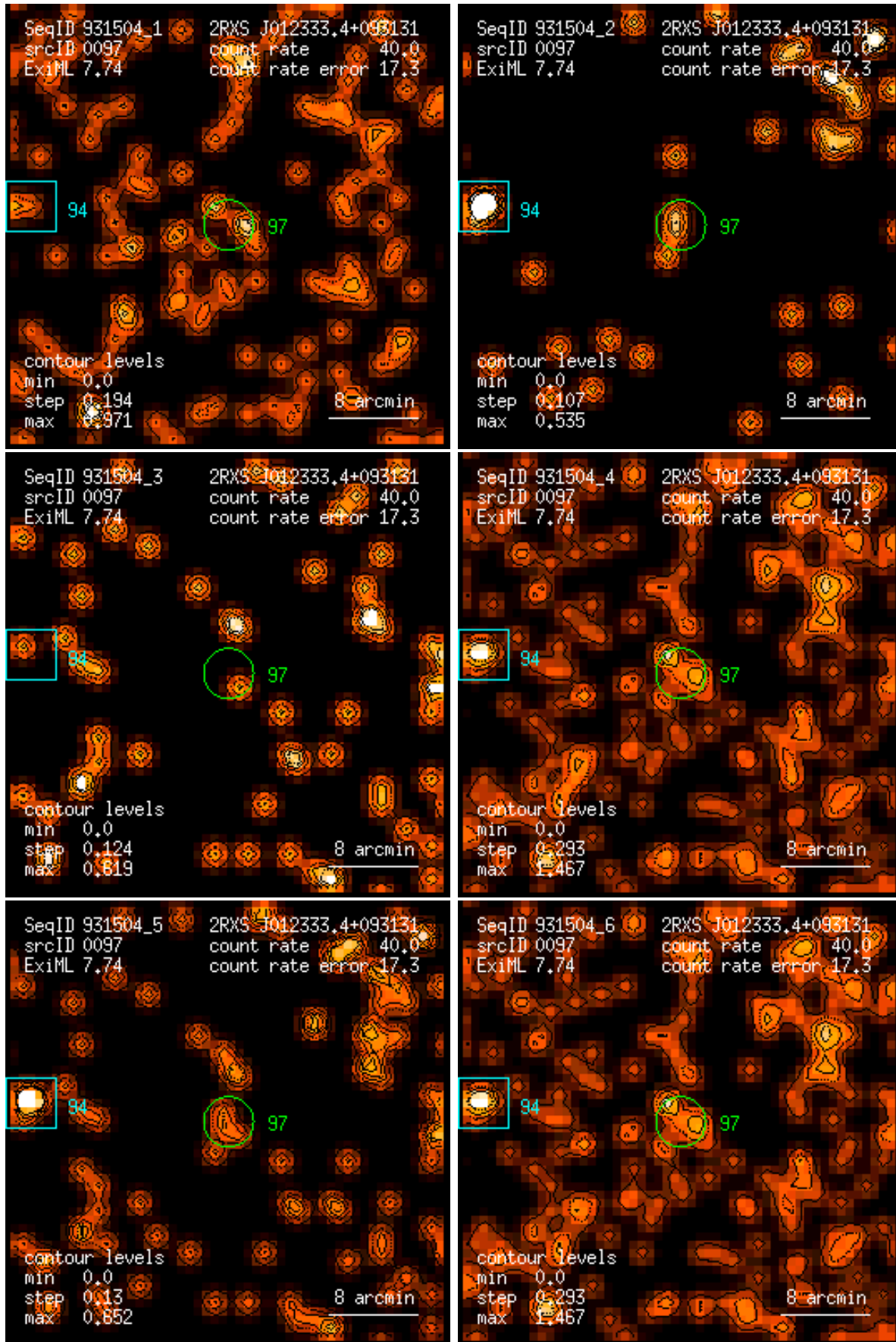
Figure 97: RASS 931504: detection 0097: band rate images, Gaussian filter: (1) PSPC channels 11 – 41, (2) 52 – 90, (3) 91 – 201, (4) 11 – 235, (5) 52 – 201, (6) 11 – 201. Broad band rates in counts/ks. Band rate contour levels in counts/ks/arcmin 2 .
