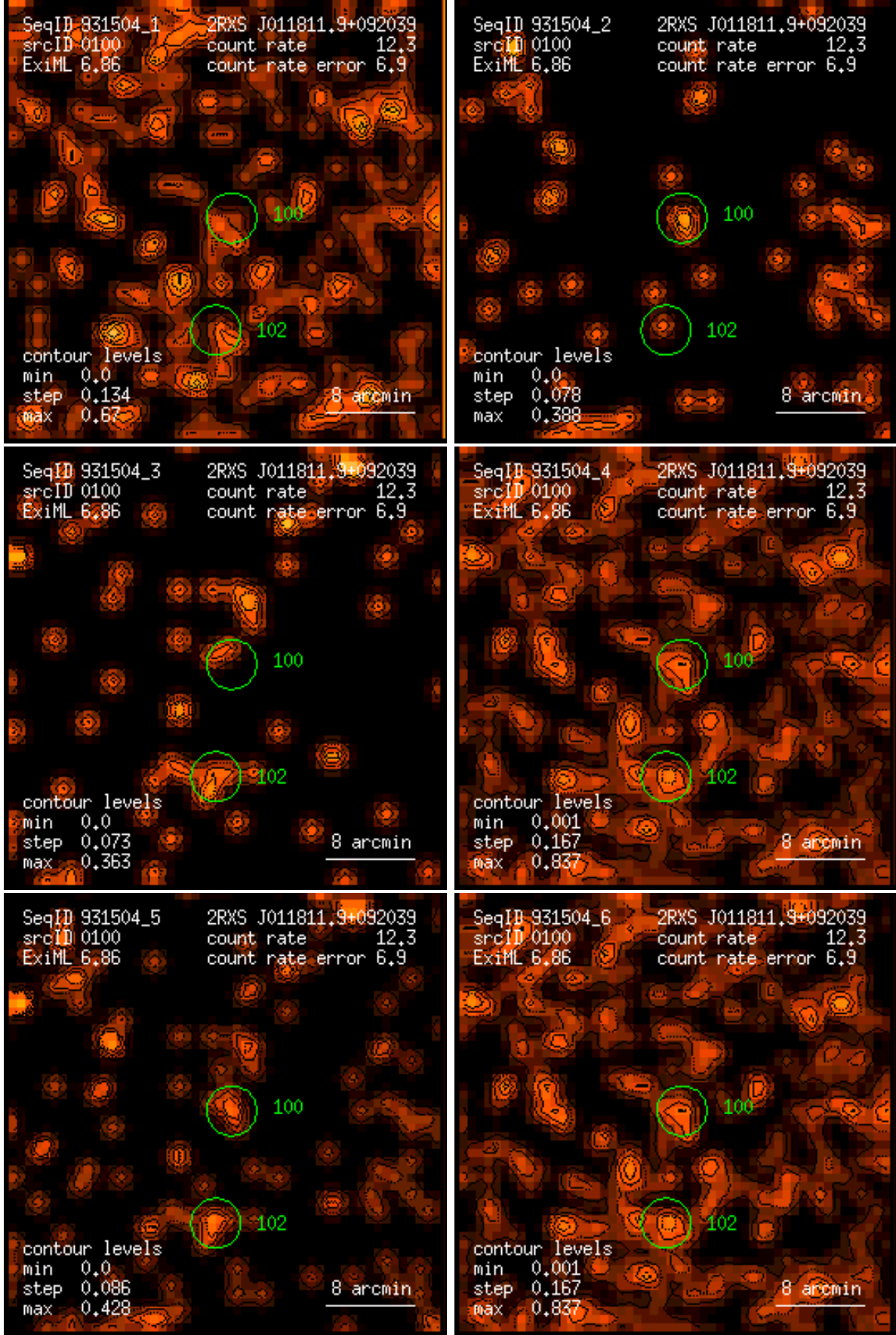
Figure 100: RASS 931504: detection 0100: band rate images, Gaussian filter: (1) PSPC channels 11 – 41, (2) 52 – 90, (3) 91 – 201, (4) 11 – 235, (5) 52 – 201, (6) 11 – 201. Broad band rates in counts/ks. Band rate contour levels in counts/ks/arcmin 2 .
