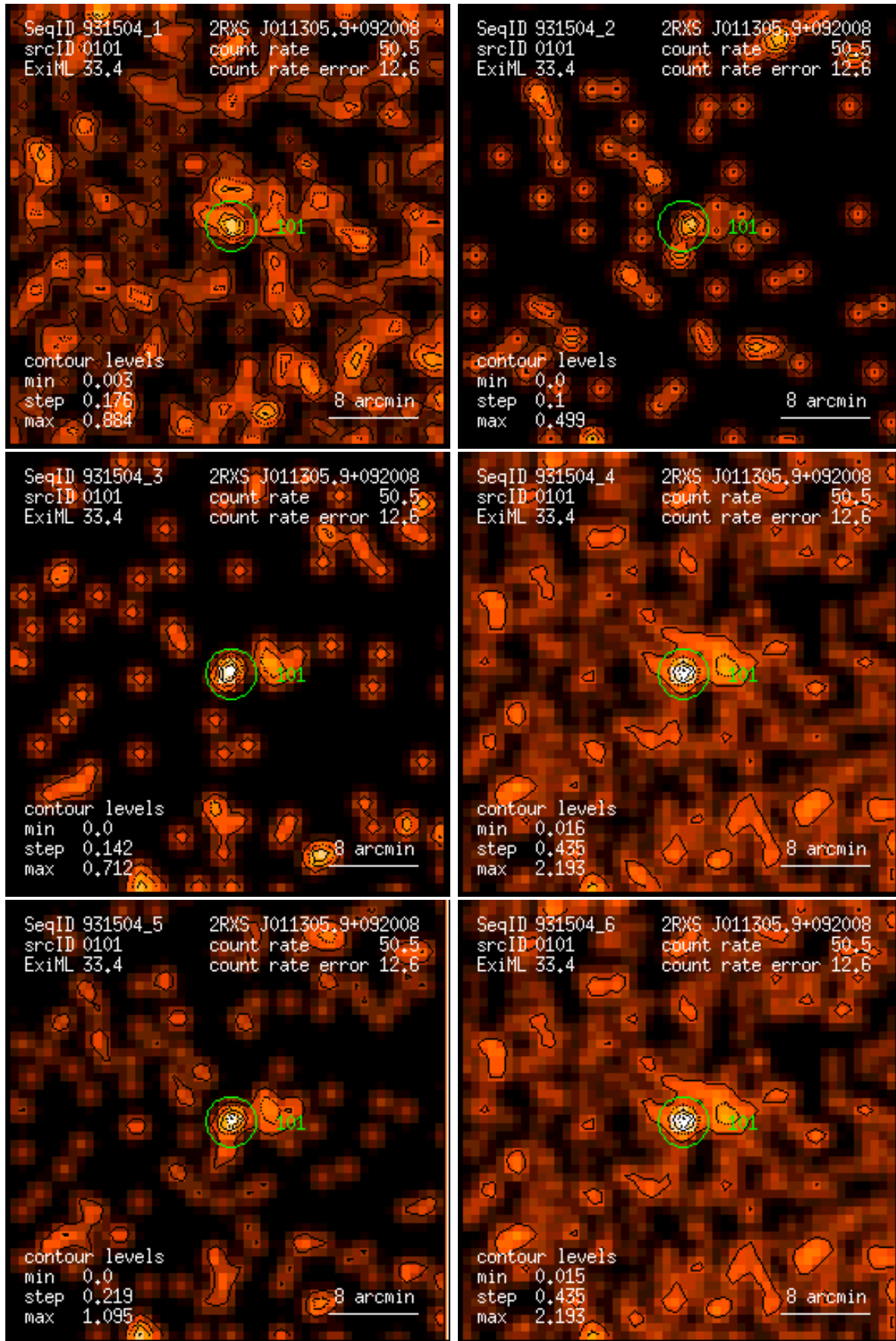
Figure 101: RASS 931504: detection 0101: band rate images, Gaussian filter: (1) PSPC channels 11 – 41, (2) 52 – 90, (3) 91 – 201, (4) 11 – 235, (5) 52 – 201, (6) 11 – 201. Broad band rates in counts/ks. Band rate contour levels in counts/ks/arcmin 2 .
