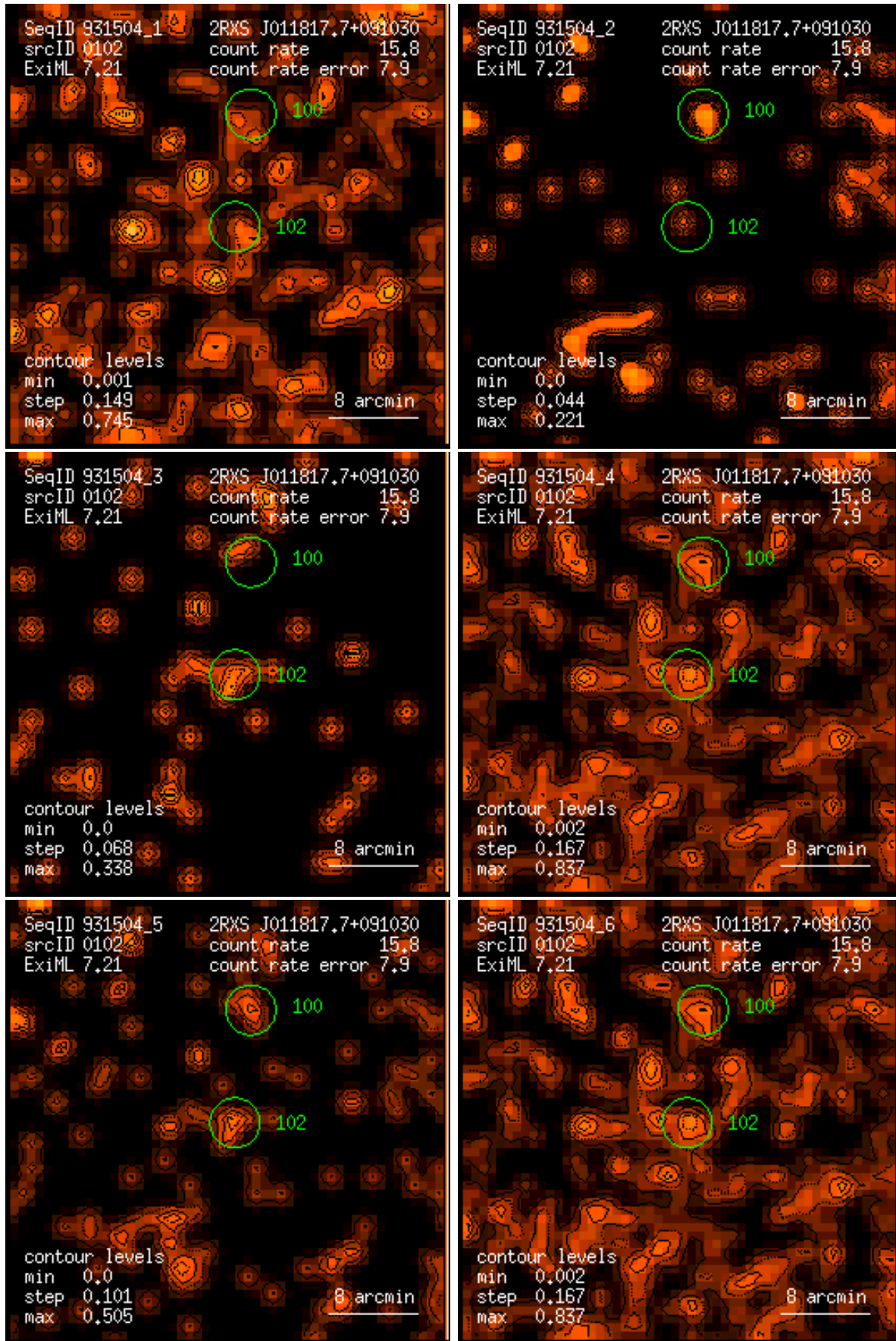
Figure 102: RASS 931504: detection 0102: band rate images, Gaussian filter: (1) PSPC channels 11 – 41, (2) 52 – 90, (3) 91 – 201, (4) 11 – 235, (5) 52 – 201, (6) 11 – 201. Broad band rates in counts/ks. Band rate contour levels in counts/ks/arcmin 2 .
