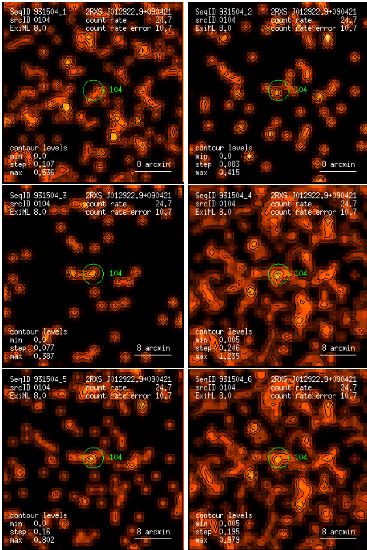
Figure 104: RASS 931504: detection 0104: band rate images, Gaussian filter: (1) PSPC channels 11 – 41, (2) 52 – 90, (3) 91 – 201, (4) 11 – 235, (5) 52 – 201, (6) 11 – 201. Broad band rates in counts/ks. Band rate contour levels in counts/ks/arcmin 2 .
