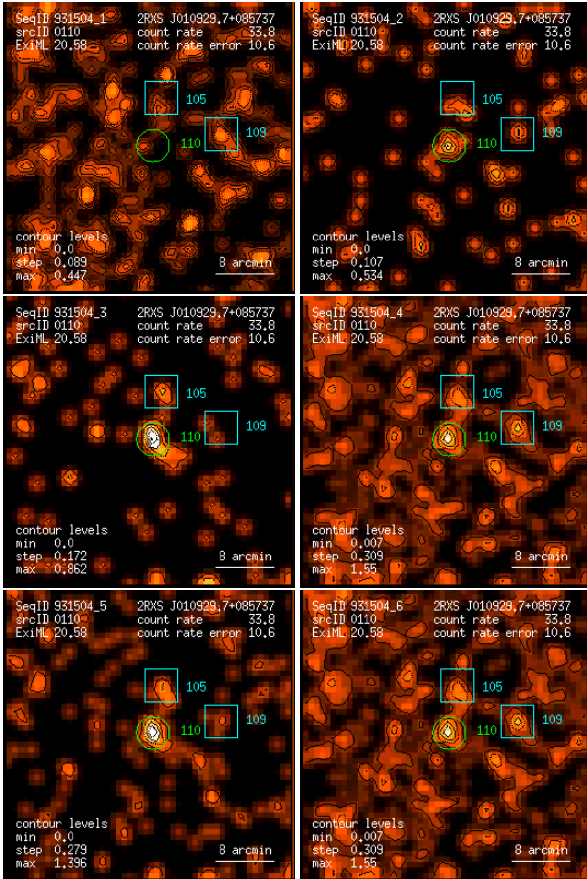
Figure 110: RASS 931504: detection 0110: band rate images, Gaussian filter: (1) PSPC channels 11 – 41, (2) 52 – 90, (3) 91 – 201, (4) 11 – 235, (5) 52 – 201, (6) 11 – 201. Broad band rates in counts/ks. Band rate contour levels in counts/ks/arcmin 2 .
