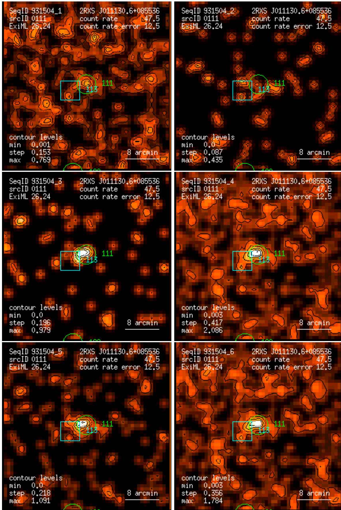
Figure 111: RASS 931504: detection 0111: band rate images, Gaussian filter: (1) PSPC channels 11 – 41, (2) 52 – 90, (3) 91 – 201, (4) 11 – 235, (5) 52 – 201, (6) 11 – 201. Broad band rates in counts/ks. Band rate contour levels in counts/ks/arcmin 2 .
