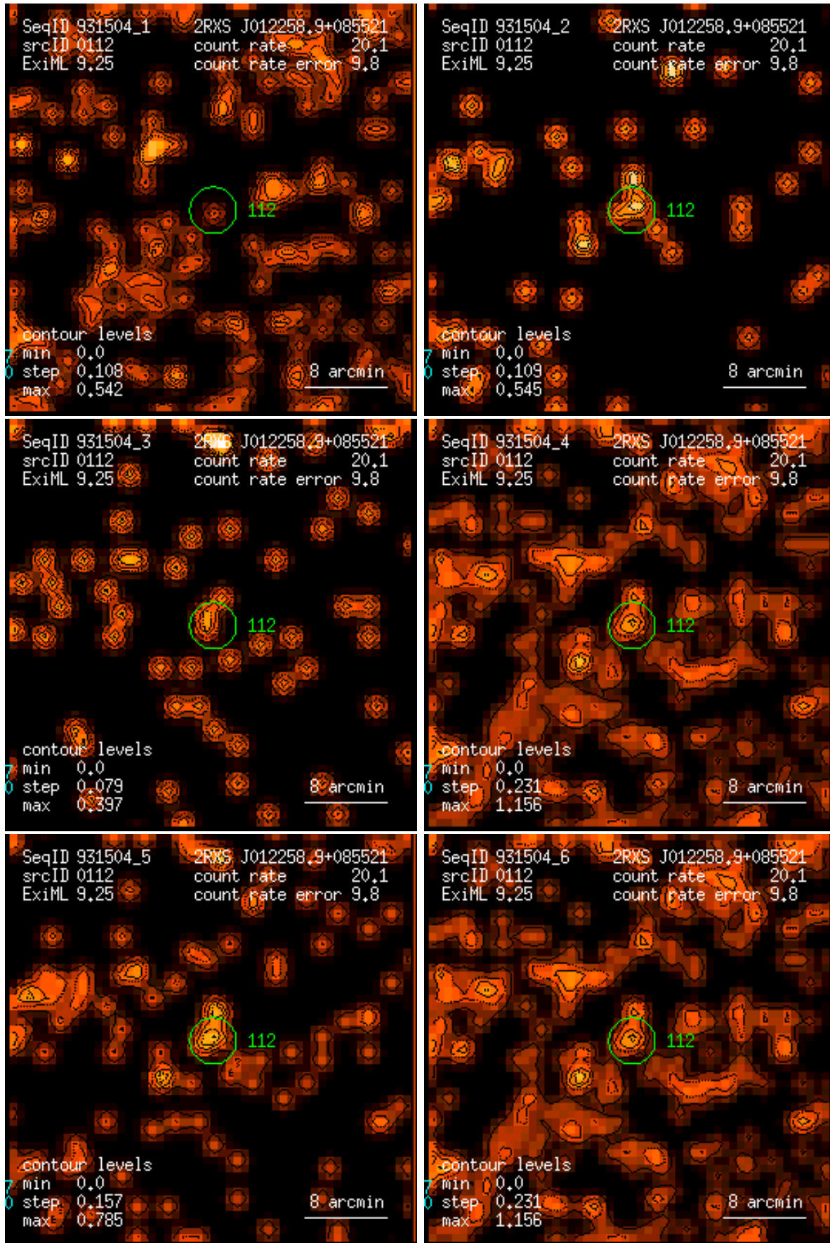
Figure 112: RASS 931504: detection 0112: band rate images, Gaussian filter: (1) PSPC channels 11 – 41, (2) 52 – 90, (3) 91 – 201, (4) 11 – 235, (5) 52 – 201, (6) 11 – 201. Broad band rates in counts/ks. Band rate contour levels in counts/ks/arcmin 2 .
