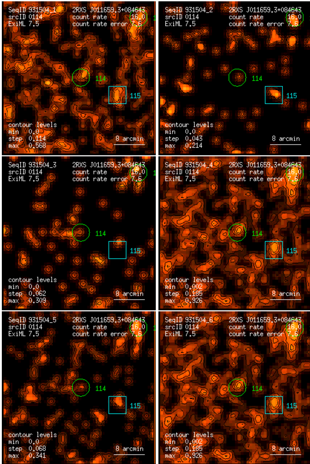
Figure 114: RASS 931504: detection 0114: band rate images, Gaussian filter: (1) PSPC channels 11 – 41, (2) 52 – 90, (3) 91 – 201, (4) 11 – 235, (5) 52 – 201, (6) 11 – 201. Broad band rates in counts/ks. Band rate contour levels in counts/ks/arcmin 2 .
