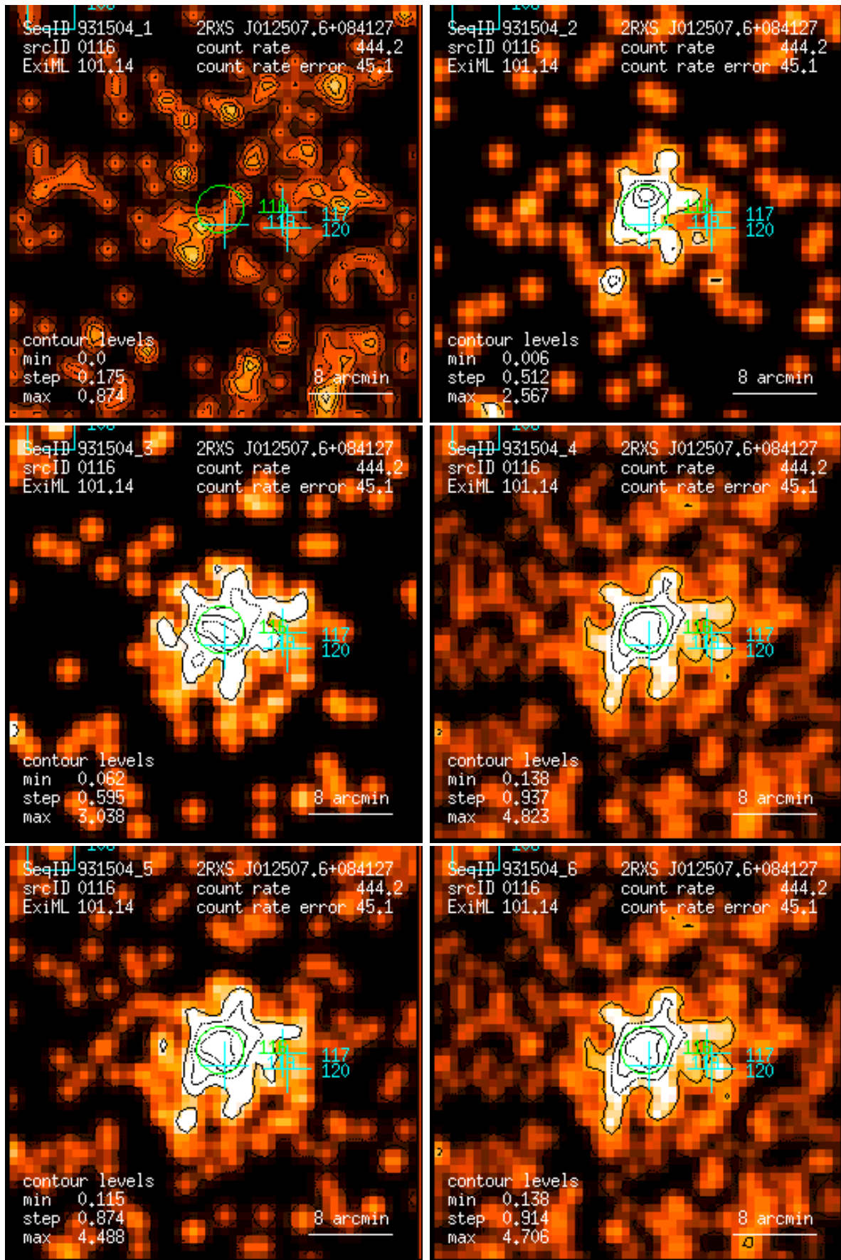
Figure 116: RASS 931504: detection 0116: band rate images, Gaussian filter: (1) PSPC channels 11 – 41, (2) 52 – 90, (3) 91 – 201, (4) 11 – 235, (5) 52 – 201, (6) 11 – 201. Broad band rates in counts/ks. Band rate contour levels in counts/ks/arcmin 2 .
