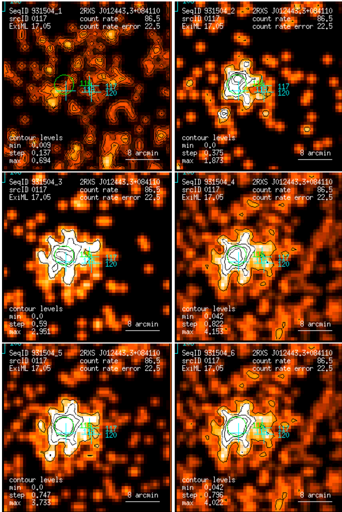
Figure 117: RASS 931504: detection 0117: band rate images, Gaussian filter: (1) PSPC channels 11 – 41, (2) 52 – 90, (3) 91 – 201, (4) 11 – 235, (5) 52 – 201, (6) 11 – 201. Broad band rates in counts/ks. Band rate contour levels in counts/ks/arcmin 2 .
