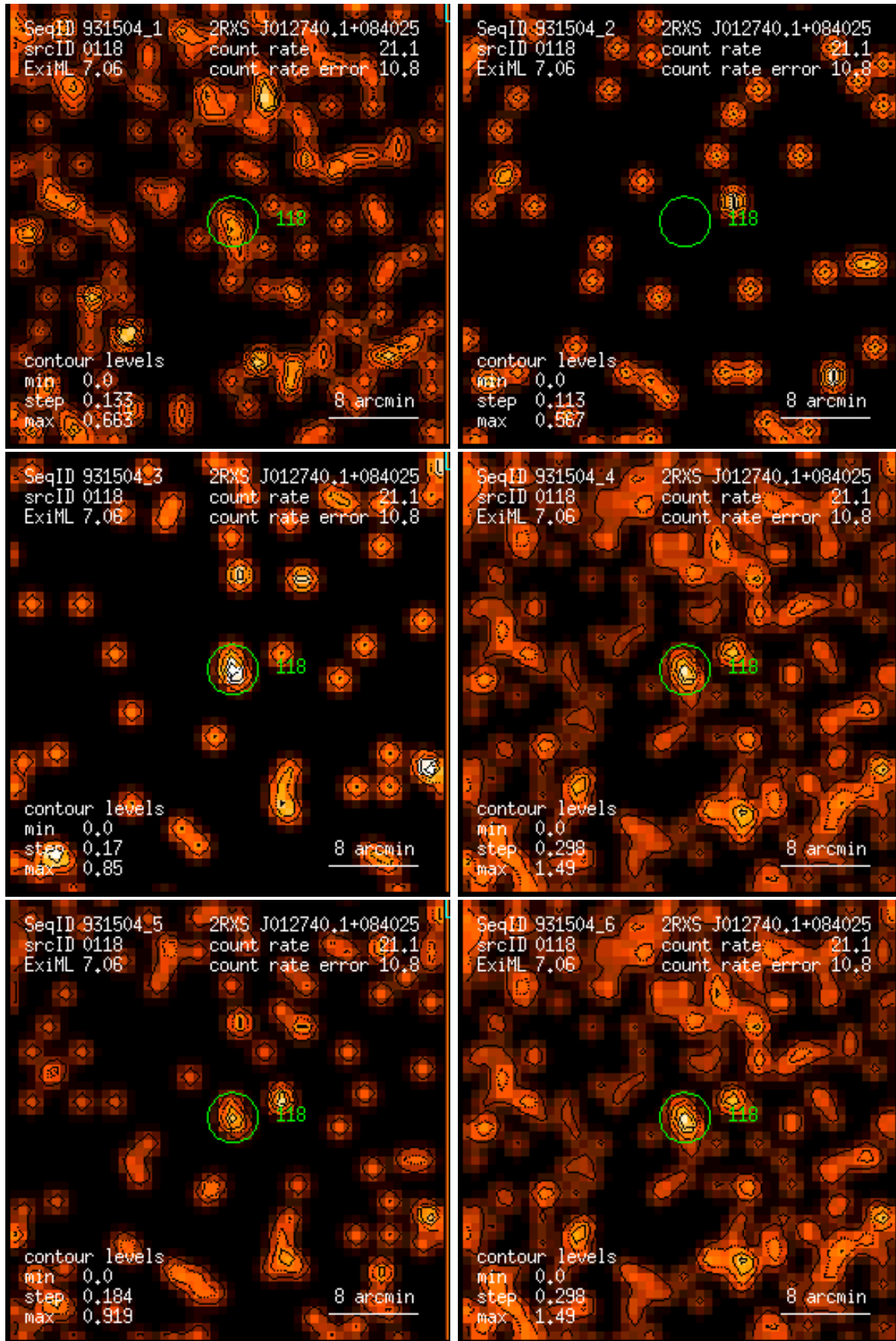
Figure 118: RASS 931504: detection 0118: band rate images, Gaussian filter: (1) PSPC channels 11 – 41, (2) 52 – 90, (3) 91 – 201, (4) 11 – 235, (5) 52 – 201, (6) 11 – 201. Broad band rates in counts/ks. Band rate contour levels in counts/ks/arcmin 2 .
