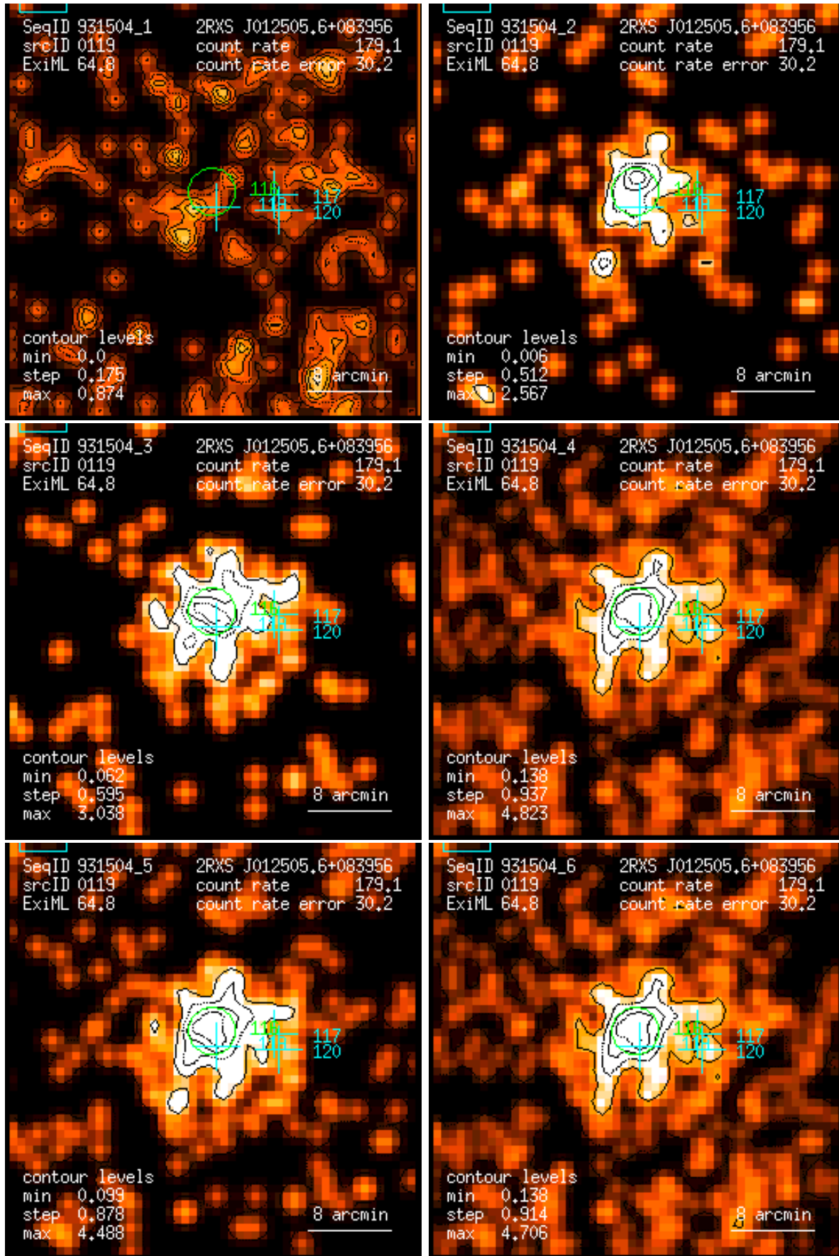
Figure 119: RASS 931504: detection 0119: band rate images, Gaussian filter: (1) PSPC channels 11 – 41, (2) 52 – 90, (3) 91 – 201, (4) 11 – 235, (5) 52 – 201, (6) 11 – 201. Broad band rates in counts/ks. Band rate contour levels in counts/ks/arcmin 2 .
