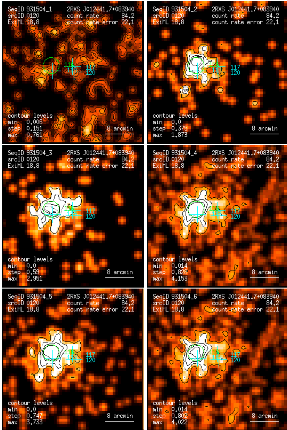
Figure 120: RASS 931504: detection 0120: band rate images, Gaussian filter: (1) PSPC channels 11 – 41, (2) 52 – 90, (3) 91 – 201, (4) 11 – 235, (5) 52 – 201, (6) 11 – 201. Broad band rates in counts/ks. Band rate contour levels in counts/ks/arcmin 2 .
