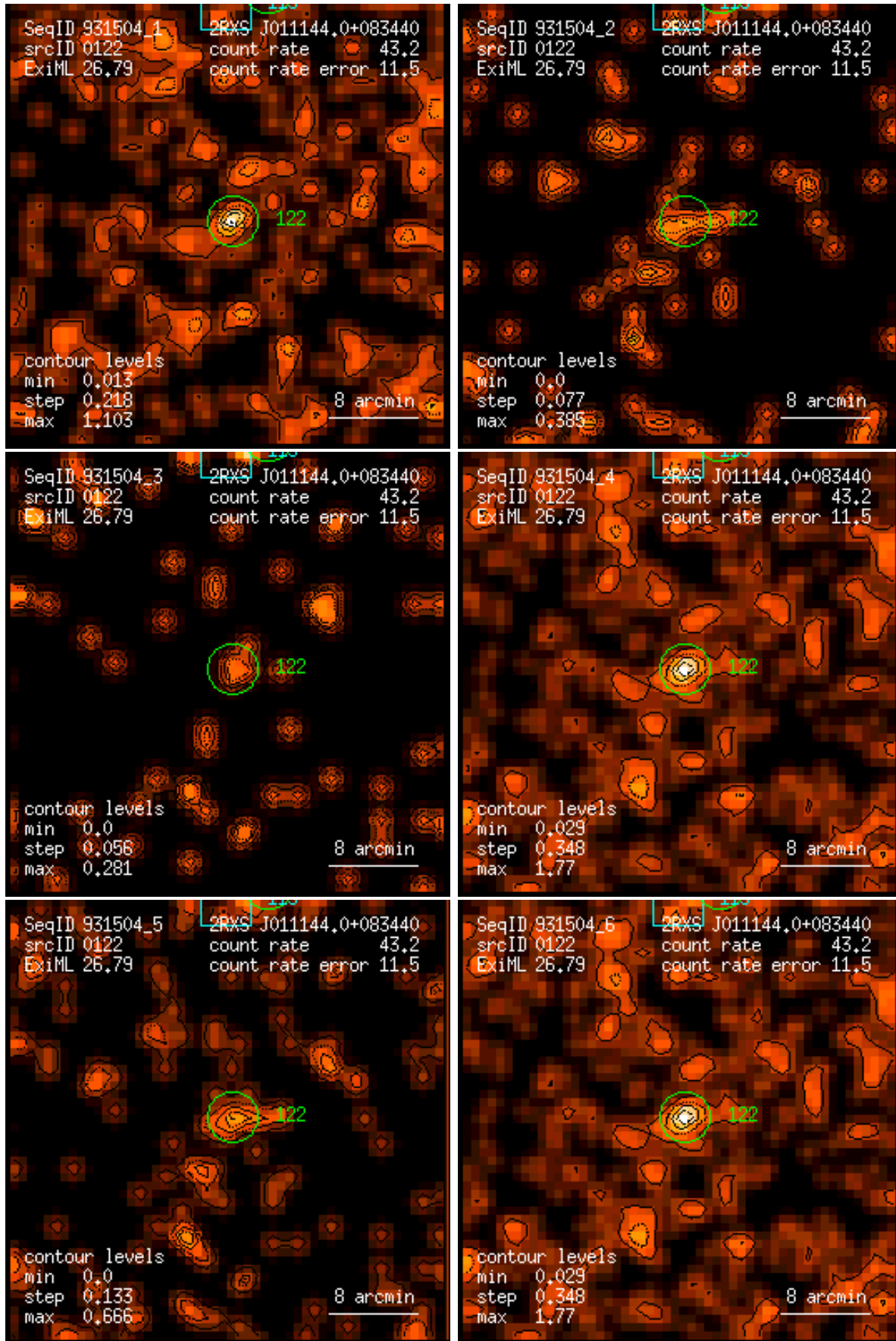
Figure 122: RASS 931504: detection 0122: band rate images, Gaussian filter: (1) PSPC channels 11 – 41, (2) 52 – 90, (3) 91 – 201, (4) 11 – 235, (5) 52 – 201, (6) 11 – 201. Broad band rates in counts/ks. Band rate contour levels in counts/ks/arcmin 2 .
