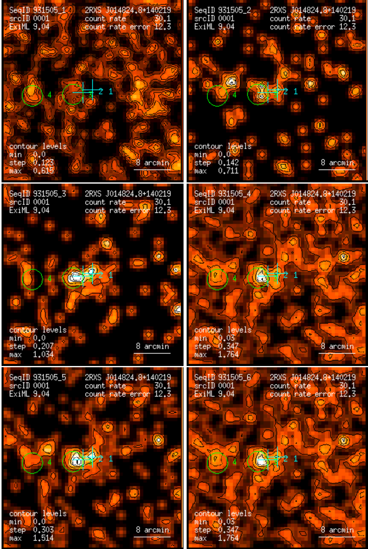
Figure 1: RASS 931505: detection 0001: band rate images, Gaussian filter: (1) PSPC channels 11 – 41, (2) 52 – 90, (3) 91 – 201, (4) 11 – 235, (5) 52 – 201, (6) 11 – 201. Broad band rates in counts/ks. Band rate contour levels in counts/ks/arcmin 2 .
