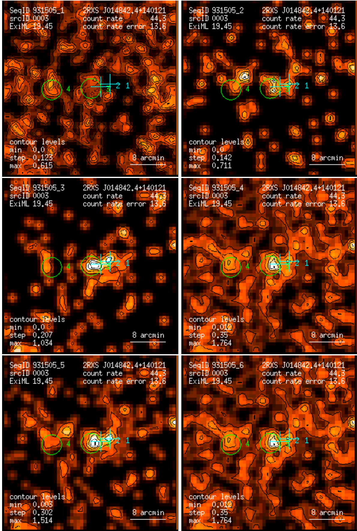
Figure 3: RASS 931505: detection 0003: band rate images, Gaussian filter: (1) PSPC channels 11 – 41, (2) 52 – 90, (3) 91 – 201, (4) 11 – 235, (5) 52 – 201, (6) 11 – 201. Broad band rates in counts/ks. Band rate contour levels in counts/ks/arcmin 2 .
