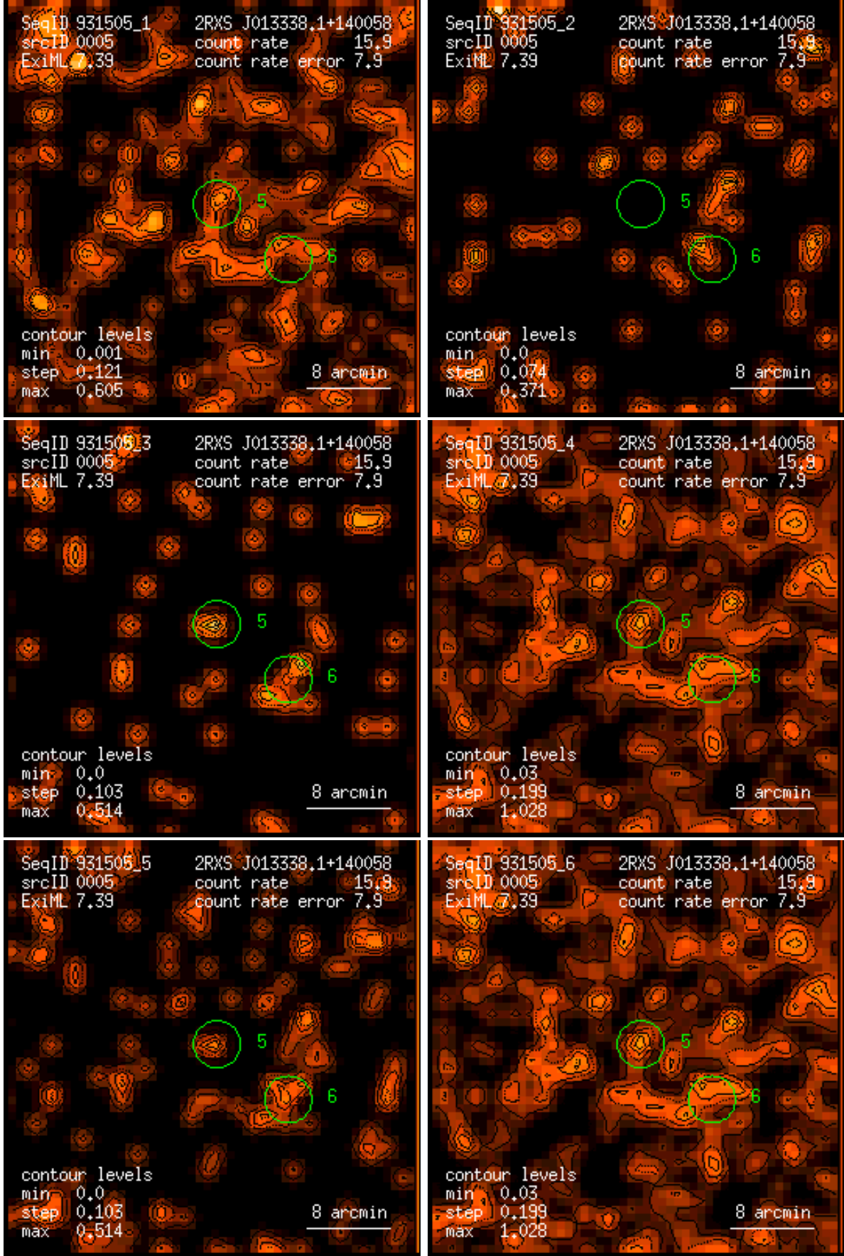
Figure 5: RASS 931505: detection 0005: band rate images, Gaussian filter: (1) PSPC channels 11 – 41, (2) 52 – 90, (3) 91 – 201, (4) 11 – 235, (5) 52 – 201, (6) 11 – 201. Broad band rates in counts/ks. Band rate contour levels in counts/ks/arcmin 2 .
